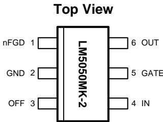
Figure 3. LM5050MK-2 SOT-6 Package
