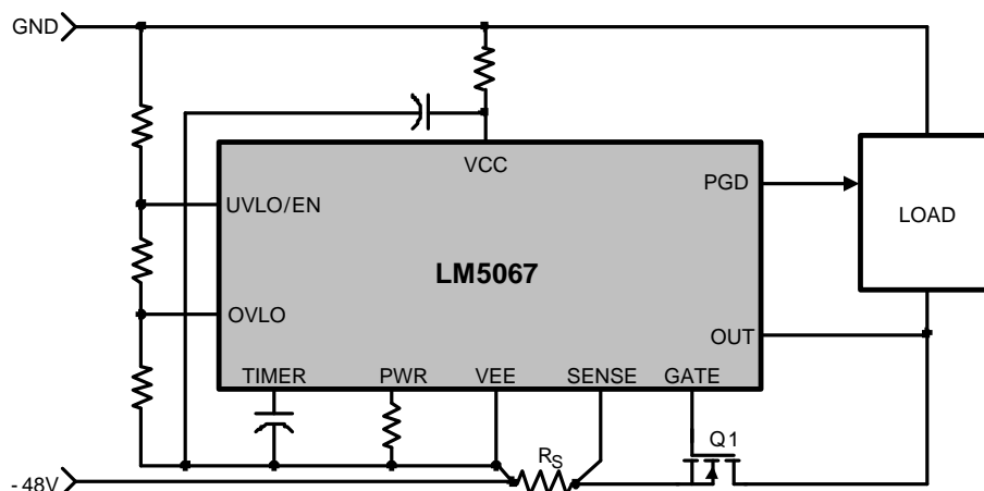
Figure 1. Negative Power Bus In-Rush and Fault Protection
