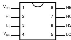
Figure 2. 8-Lead WSON See NGT0008A Package
