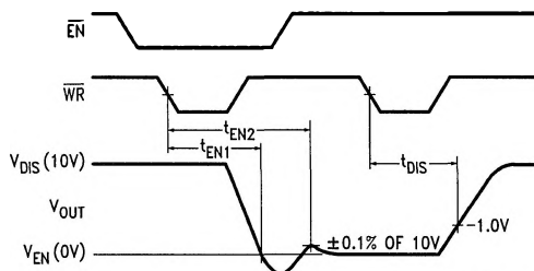
FIGURE 3. Bi-State Output Enable and Disable Time Test
