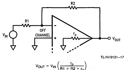
FIGURE 11. Inverting Gain Channel Feedthrough
