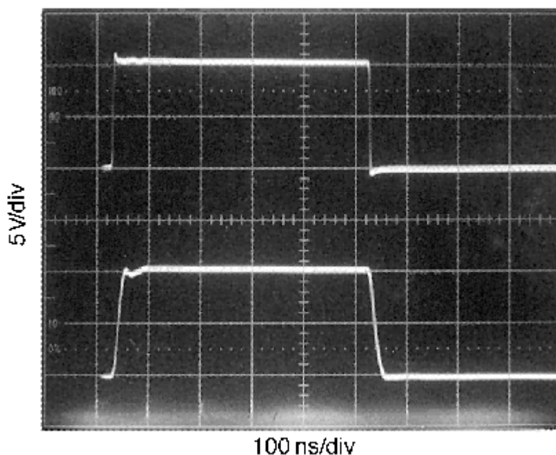
Figure 61. The LM6171 Driving a 200 pF Load with a 50Ω Isolation Resistor
