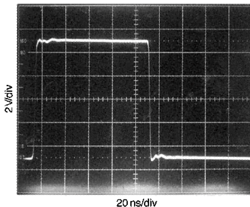
Figure 58. Properly Terminated Signal
