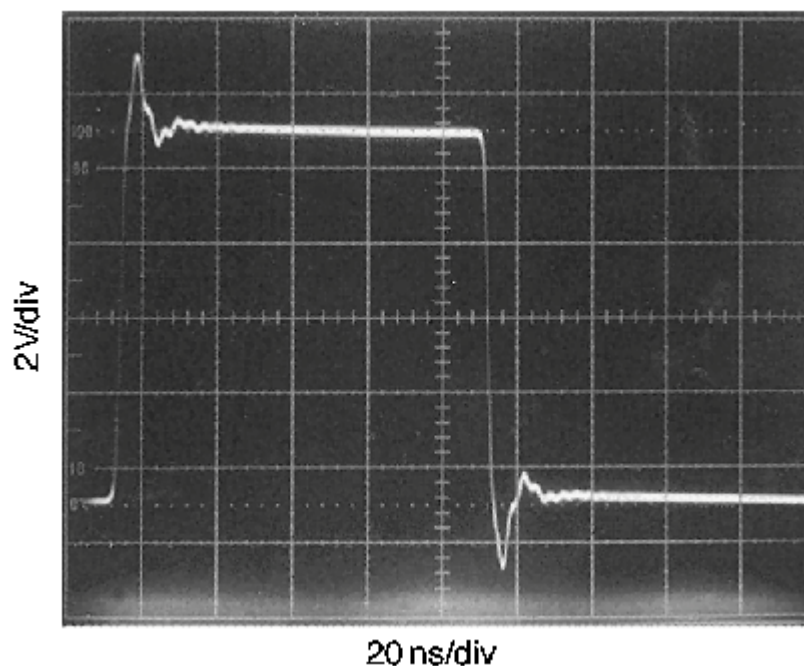
Figure 59. Improperly Terminated Signal
