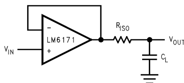
Figure 60. Isolation Resistor Used to Drive Capacitive Load
