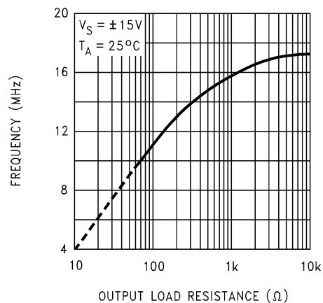
Unity Gain Bandwidth vs Output Load
