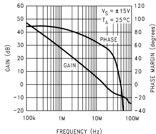
Frequency Response High Frequency
