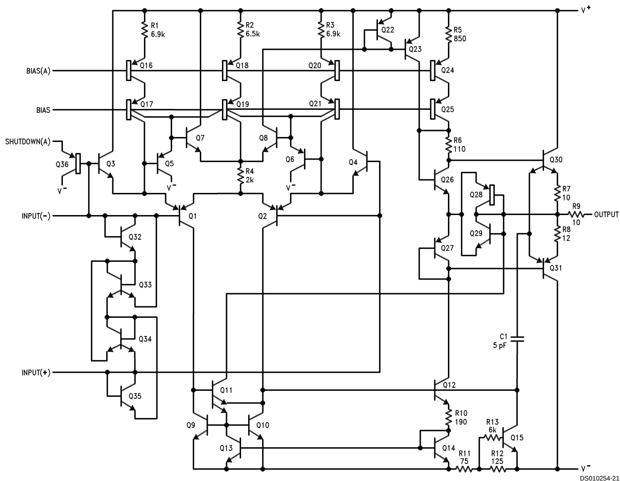
1/2 LM6118 (Op Amp A)
