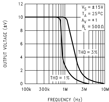
Large Signal Response (Sine Wave)
