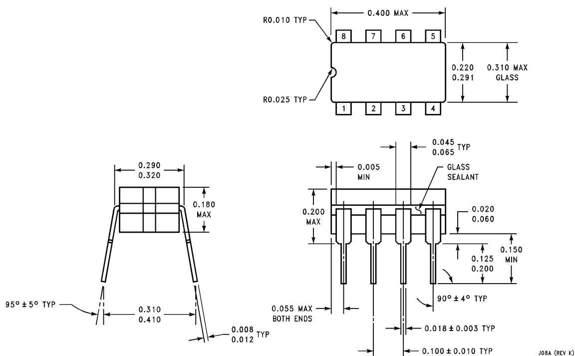
8-Lead Molded Small Outline Package (M) NS Package Number J08A
