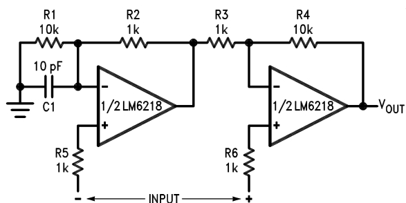
Instrumentation Amplifier
