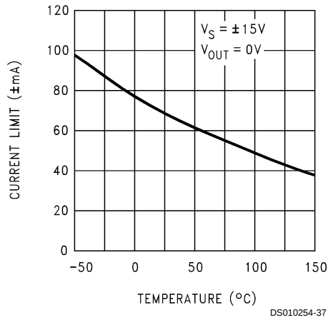
Output Current Limit
