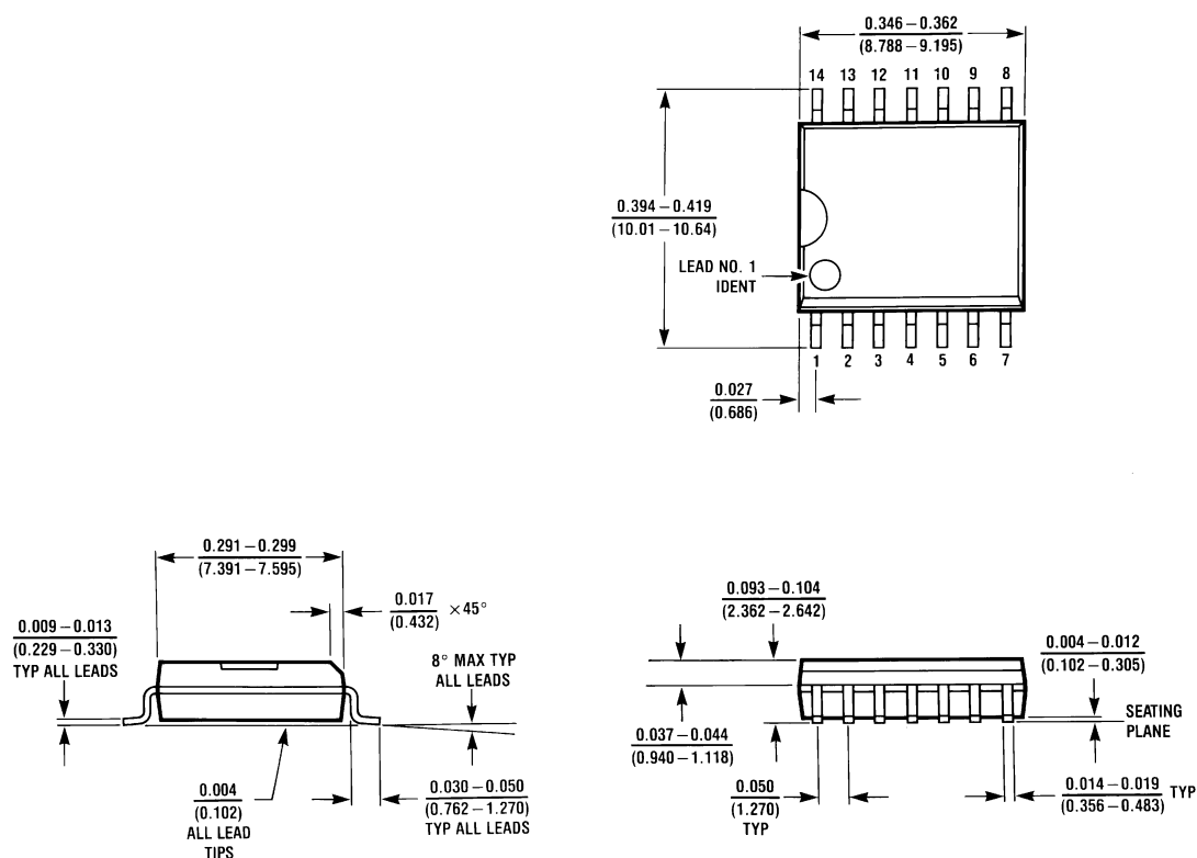
8-Lead Molded Small Outline Package (M) Order Number LM6218WM or LM6218WMX NS Package Number M14B
