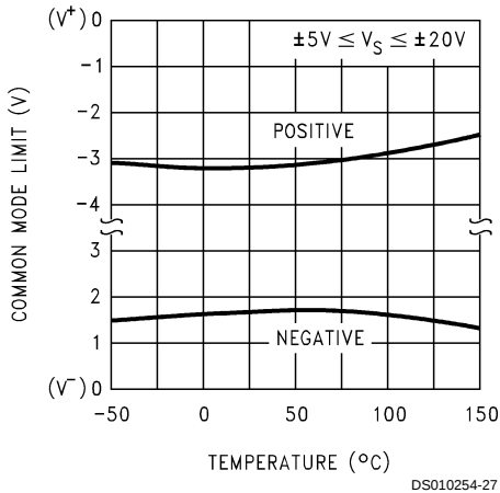
Common Mode Limits
