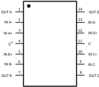
Figure 1. 14-Pin SOIC/TSSOP (Top View)
