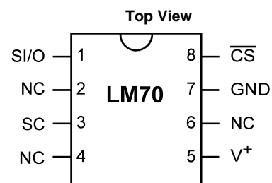
Figure 3. WSON-8 Package See Package Number NGK0008A
