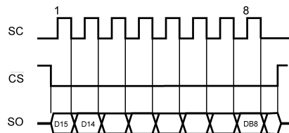
Figure 13. a) Reading Continuous Conversion - Single Eight-Bit Frame
