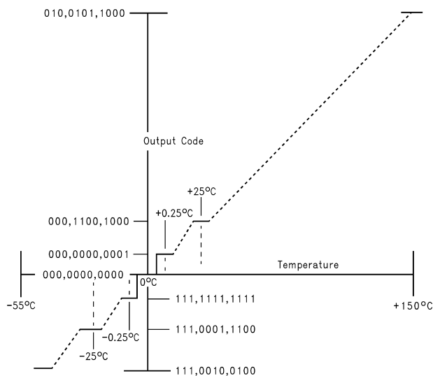
Figure 8. Temperature-to-Digital Transfer Function (Non-linear scale for clarity)
