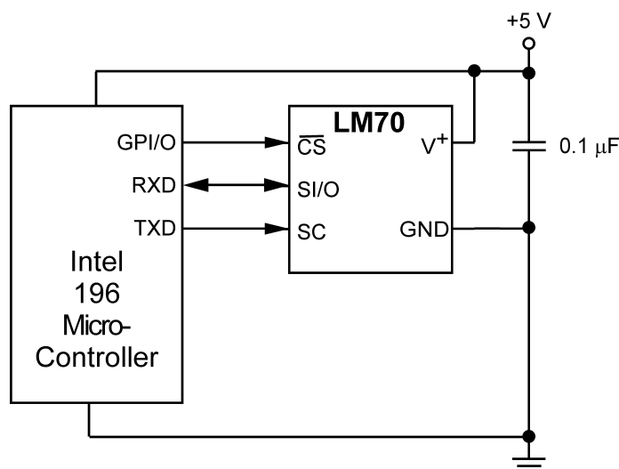
Figure 16. Temperature Monitor Using Intel 196 Processor
