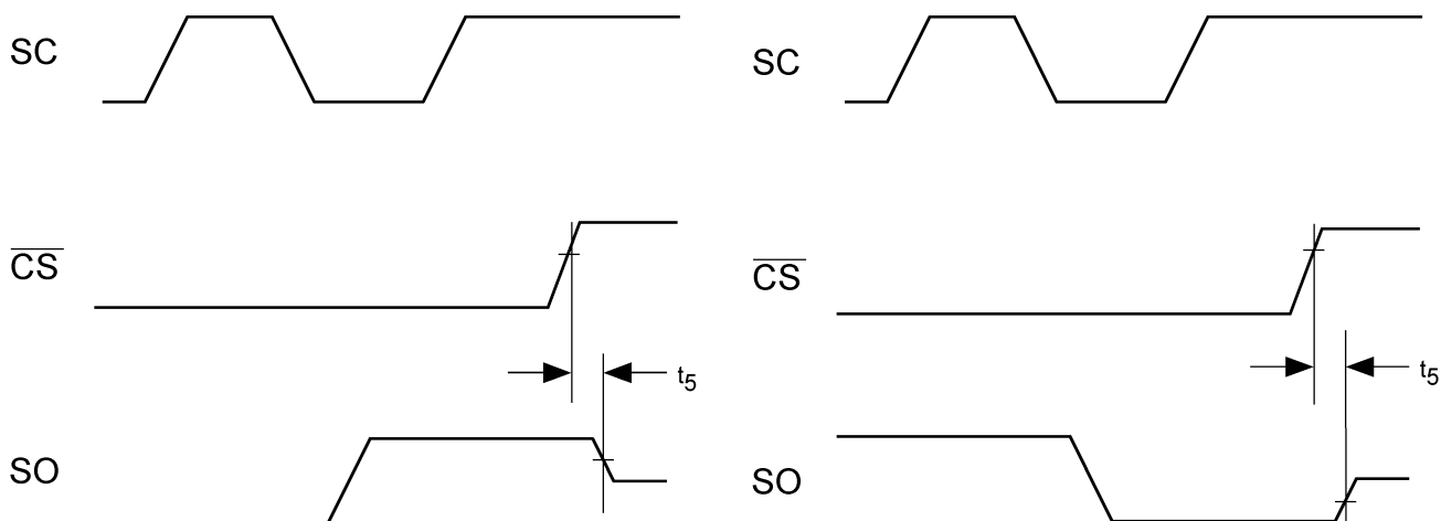
Figure 7. Data Input Timing Diagram
