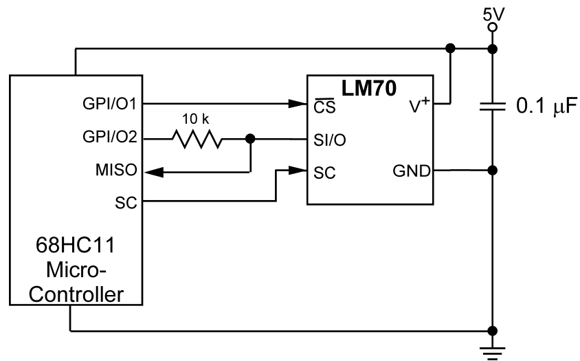
Figure 17. LM70 Digital Input Control Using Micro-Controller's General Purpose I/O
