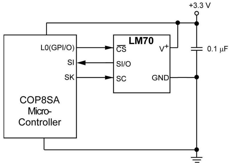
Figure 4. COP Microcontroller Interface
