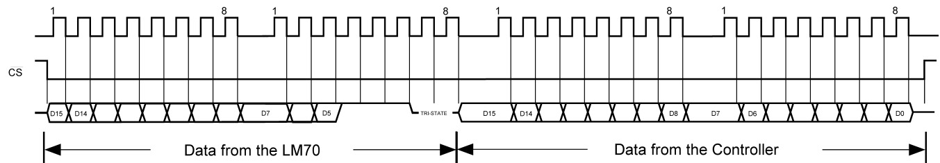
Figure 15. c) Writing Shutdown Control
