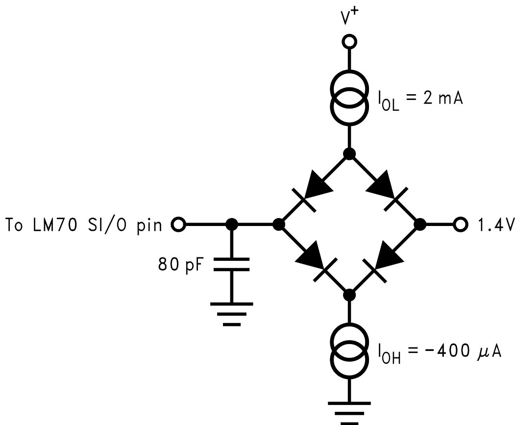
Figure 9. TRI-STATE Test Circuit
