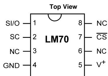
Figure 2. VSSOP-8 Package See Package Number DGK0008A
