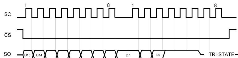
Figure 14. b) Reading Continuous Conversion - Two Eight-Bit Frames
