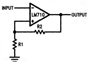
Schmitt Trigger
