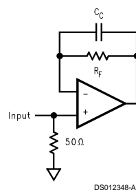
(b) A_V = +2
