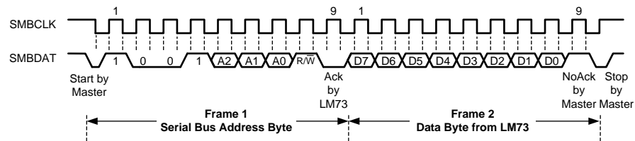
Figure 7. (c) Typical Read from a 1-Byte Register with Preset Pointer
