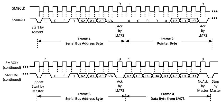
Figure 8. Reading from the LM73
