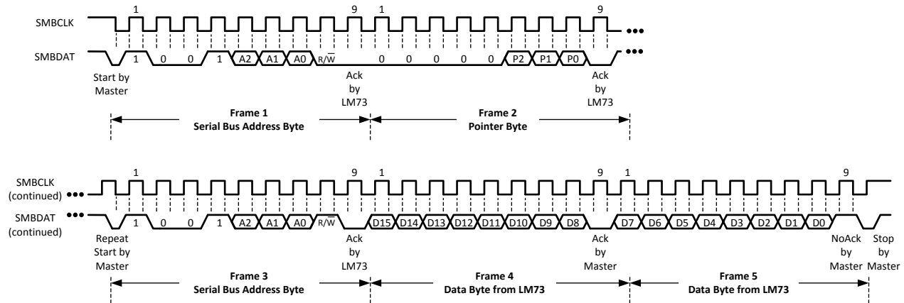
Figure 6. (b) Typical Pointer Set Followed by Immediate Read of a 2-Byte Register
