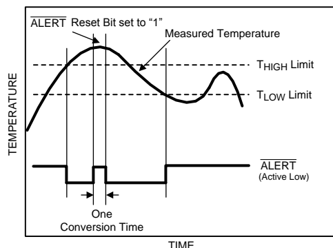
Figure 4. \overline{\text{ALERT}} Temperature Response cleared by writing a "1" to the \overline{\text{ALERT}} Reset Bit.
