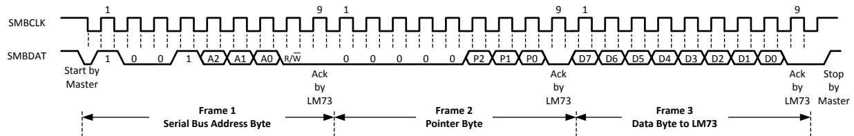
Figure 9. (a) Typical 1-Byte Write
