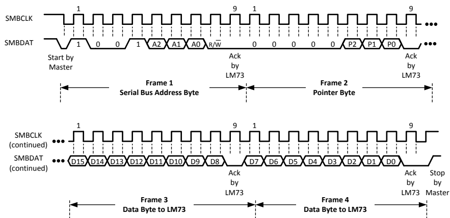
(b) Typical 2-Byte Write
