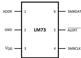
Figure 1. SOT23-6 TOP VIEW
