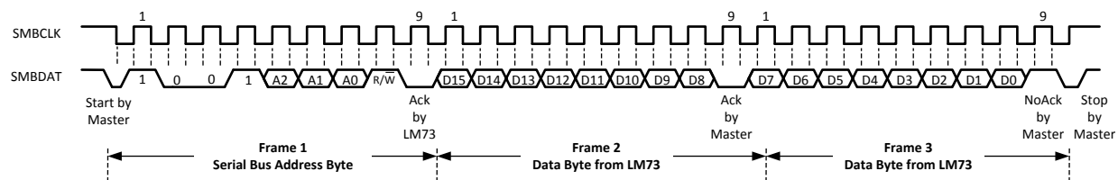
Figure 5. (a) Typical Read from a 2-Byte Register with Preset Pointer
