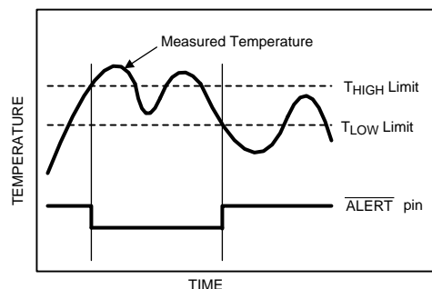
Figure 3. \overline{\text{ALERT}} Temperature Response cleared when temperature crosses T_{\text{LOW}}
