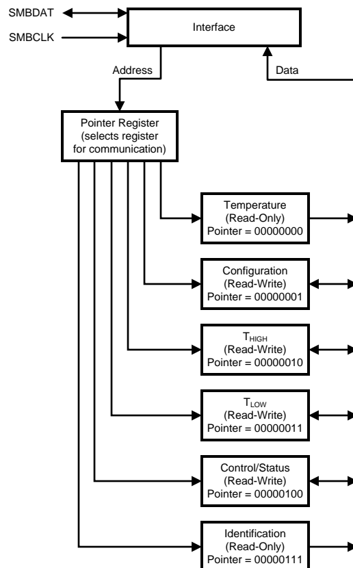
Figure 11. Pointer Register
