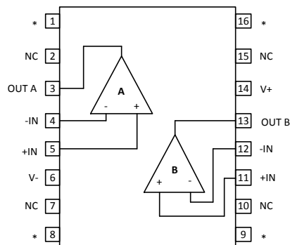
16-Pin SOIC
