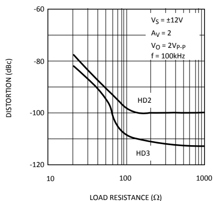
Harmonic Distortion vs. Load Resistance
