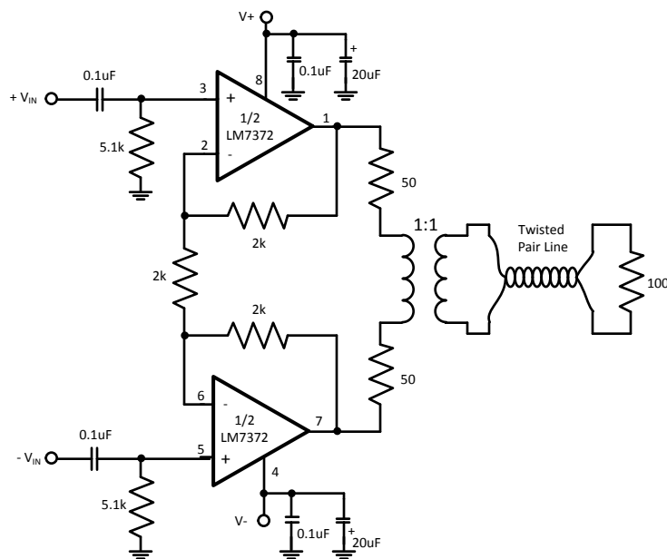
Figure 6. Split Supply Application (PSOP)
