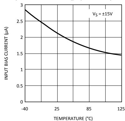
Input Bias Current (μA) vs. Temperature
