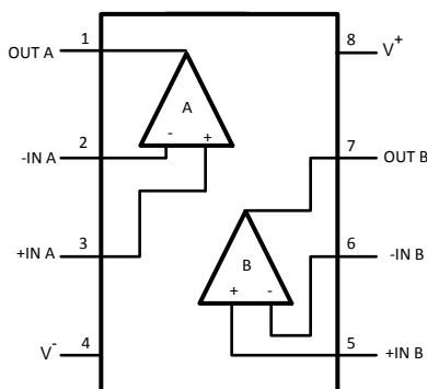
Figure 3. Top View
