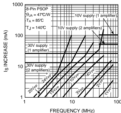
Figure 5. Power Supply Current Increase
