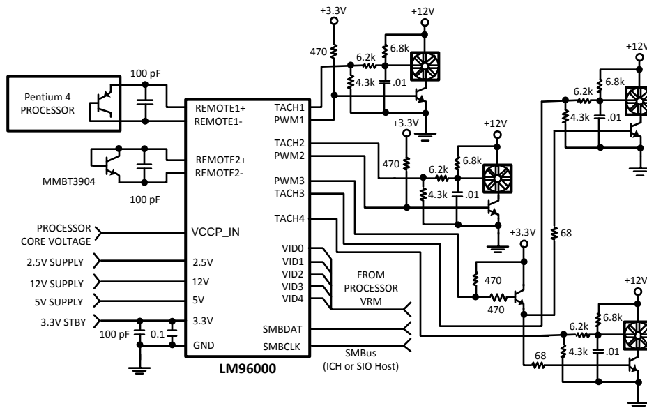
Figure 11. Typical Applications Schematic
