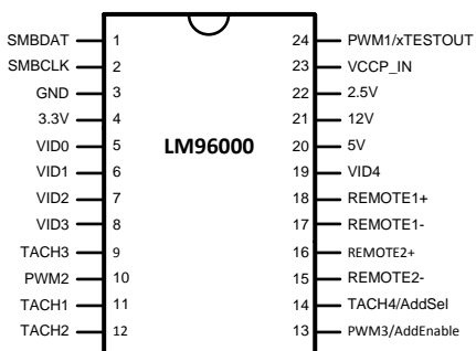
Figure 1. Package MTC24E Top View
