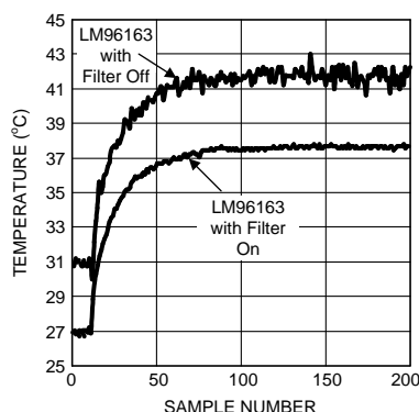
Figure 7. Digital Filter Response in a typical Intel processor on a 65 nm or 90 nm process
