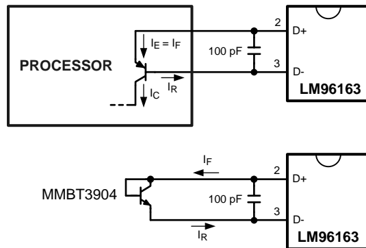
Figure 11. Thermal Diode Current Paths
