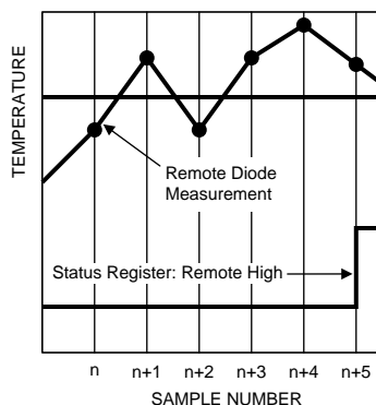
Figure 8. Fault Queue Temperature Response Diagram
