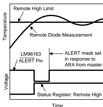
Figure 5. \overline{\text{ALERT}} Output as an SMBus ALERT Temperature Response Diagram
