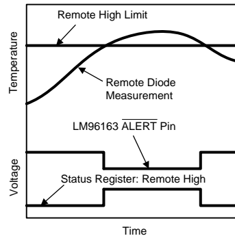
Figure 3. \overline{\text{ALERT}} Output as Temperature Comparator Response Diagram
