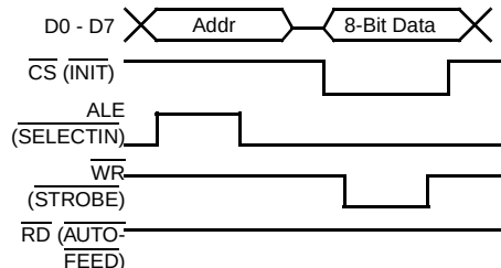
Figure 56: Writing to the Configuration Register ( \mu\text{P} )
