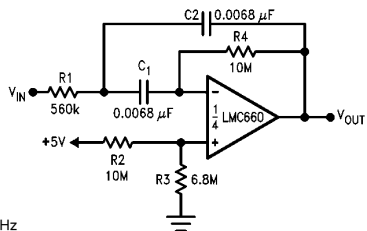
10 Hz Bandpass Filter
