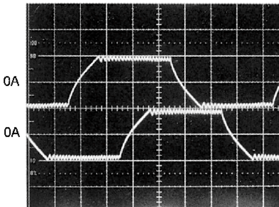
Figure 15. Winding Currents and Digital Control Signals for One-Phase-On Drive (Wave Drive)
