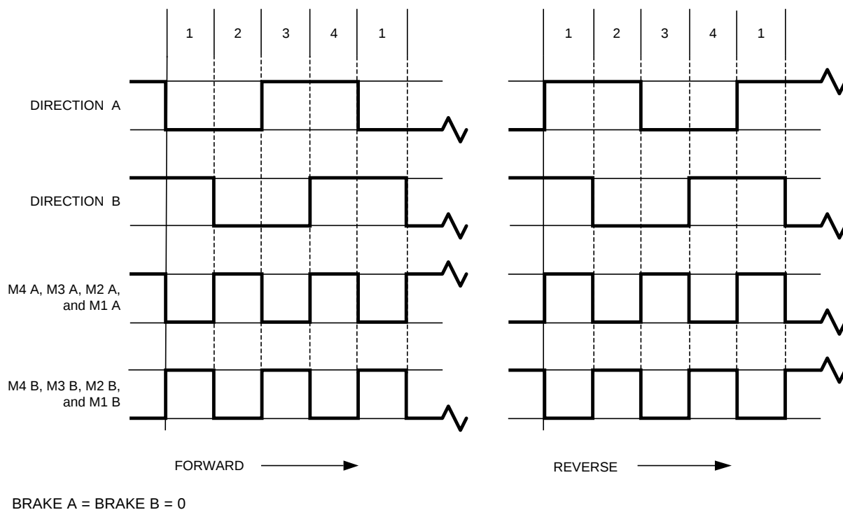
Figure 15. Winding Currents and Digital Control Signals for One-Phase-On Drive (Wave Drive)
