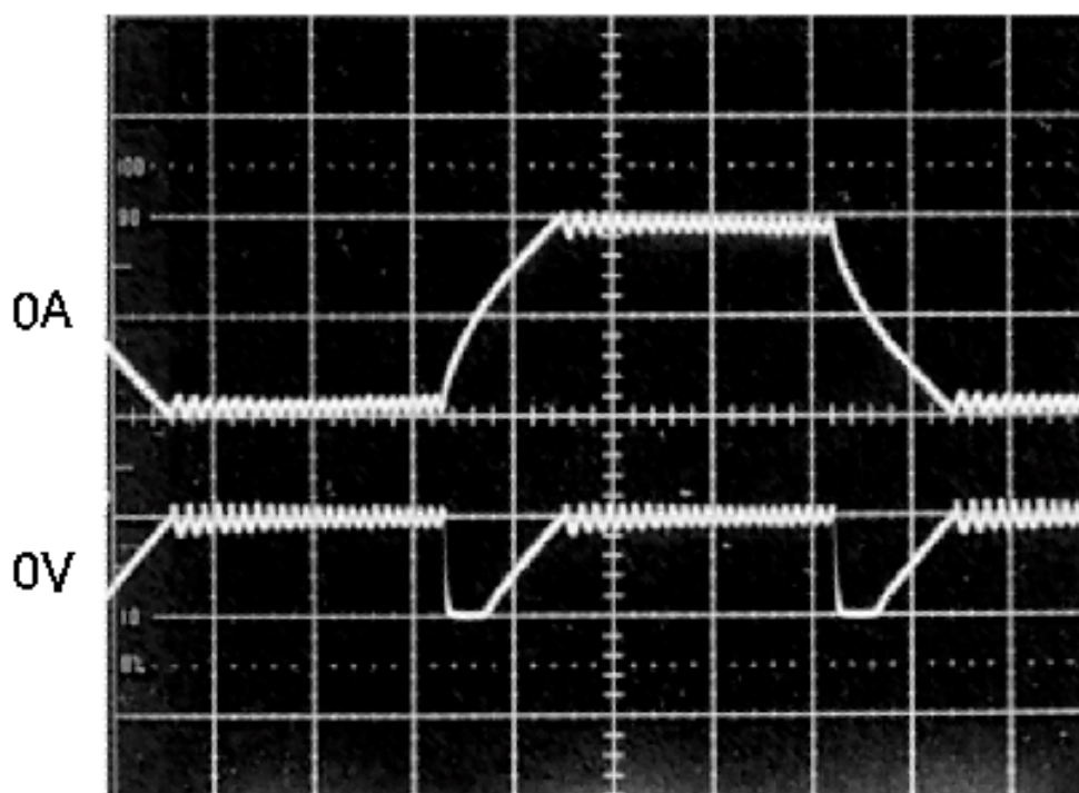
Figure 16. Winding Currents and Digital Control Signals for Two-Phase-On Drive
