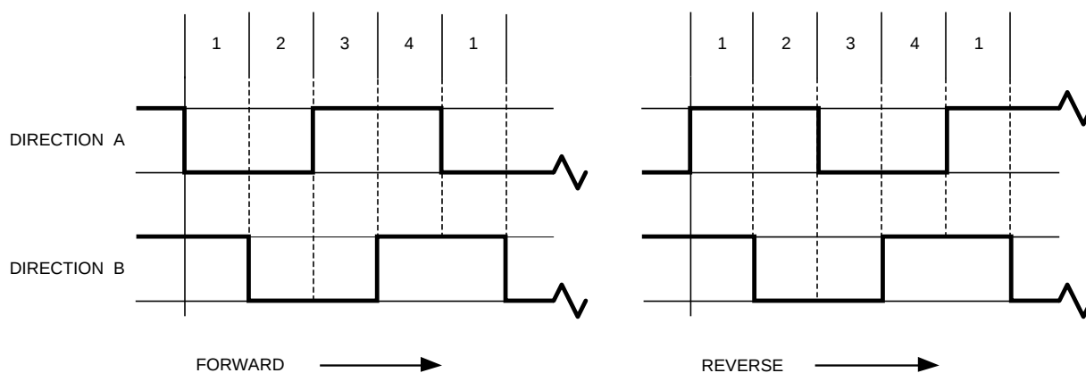
Figure 16. Winding Currents and Digital Control Signals for Two-Phase-On Drive
