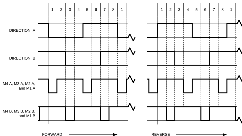
Figure 18. Winding Currents and Digital Control Signals for Half Step Drive without Torque Compensation
