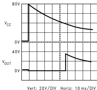
Figure 20. Overtolerance/Undervoltage Shutdown
