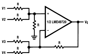
Figure 12. Adder/Subtractor
