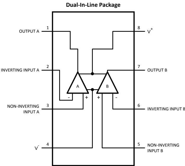
Figure 2. Dual-In-Line Package
