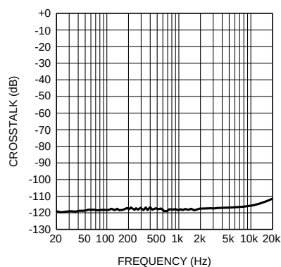
Crosstalk vs Frequency V CC = 15V, V EE = -15V, V OUT = 3V RMS A V = 0dB, R L = 2kΩ
