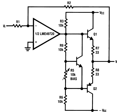
Figure 19. Line Driver
