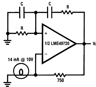
Figure 13. Sine Wave Oscillator
