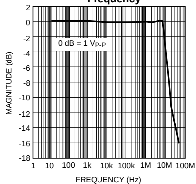
Full Power Bandwidth vs Frequency
