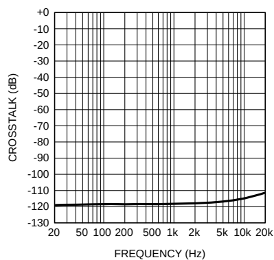
Crosstalk vs Frequency V CC = 15V, V EE = -15V, V OUT = 10V RMS A V = 0dB, R L = 2kΩ
