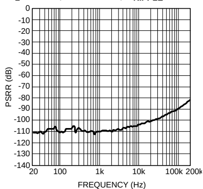
PSRR+ vs Frequency V_{CC} = 2.5V , V_{EE} = -2.5V R_L = 600\Omega , f = 200kHz , V_{RIPPLE} = 200mV_{pp}
