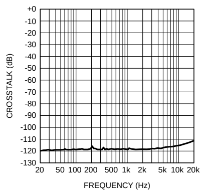
Crosstalk vs Frequency V CC = 12V, V EE = -12V, V OUT = 3V RMS A V = 0dB, R L = 2kΩ
