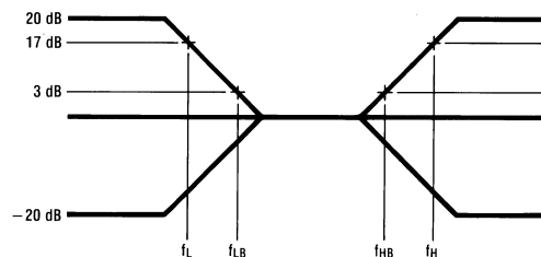
Figure 20. Tone Control
