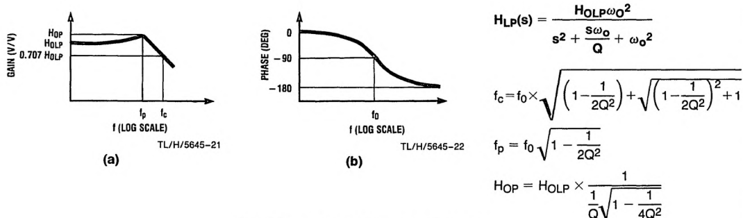
FIGURE 2. 2nd-Order Low-Pass Response
