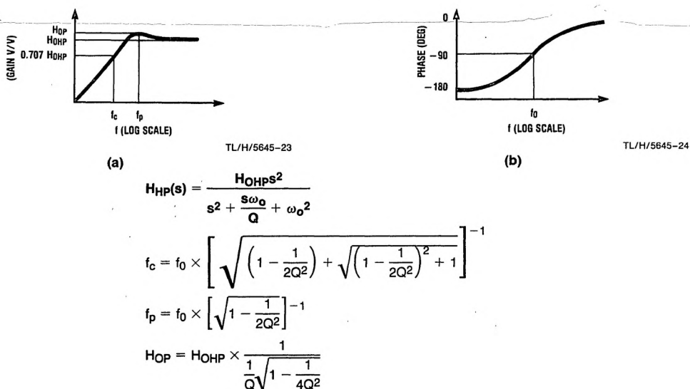
FIGURE 3. 2nd-Order High-Pass Response
