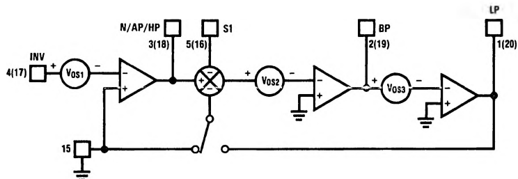
FIGURE 22. Offset Voltage Sources
