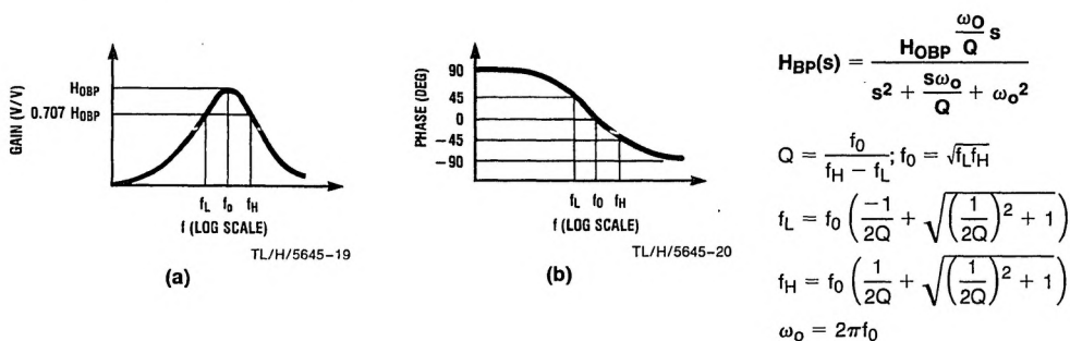
FIGURE 1. 2nd-Order Bandpass Response
