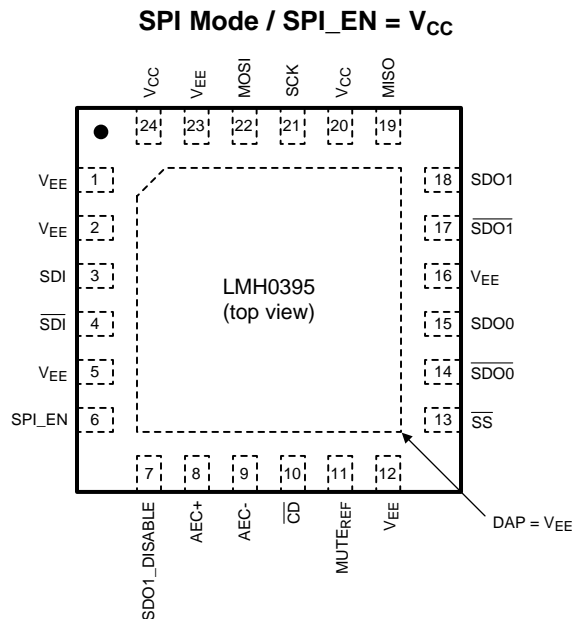
Figure 2. 24-Pin LLP
