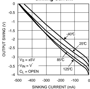
Negative Output Swing vs. Sinking Current
