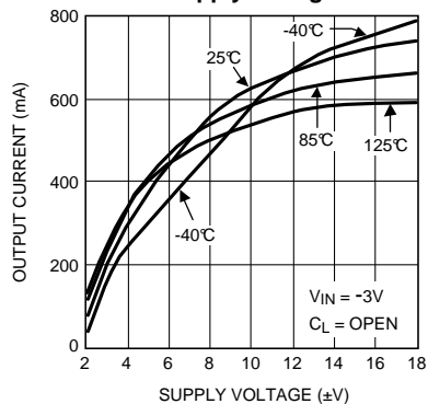
Output Short Circuit Current—Sinking vs. Supply Voltage
