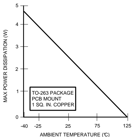
Figure 7. Derating Curve for TO-263 package. No Air Flow
