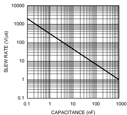
Figure 10. Slew Rate vs. Load Capacitance
