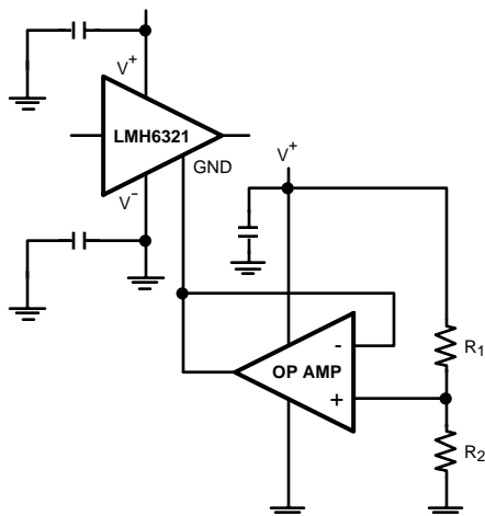
Figure 8. Using an Op Amp to Bias the GND Pin to \frac{1}{2} V^+ for Single Supply Operation
