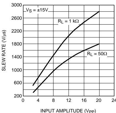
Figure 9. Slew Rate vs. Peak-to-Peak Input Voltage
