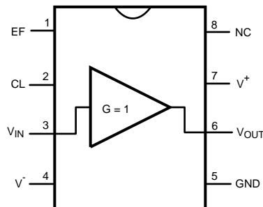
Figure 1. 8-Pin PSOP
