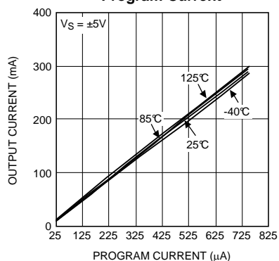
Output Short Circuit Current—Sinking vs. Program Current
