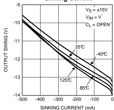
Negative Output Swing vs. Sinking Current
