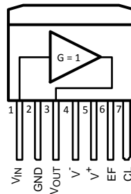
Figure 2. 7-Pin TO-263 (A)
