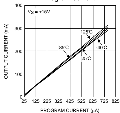
Output Short Circuit Current—Sourcing vs. Program Current
