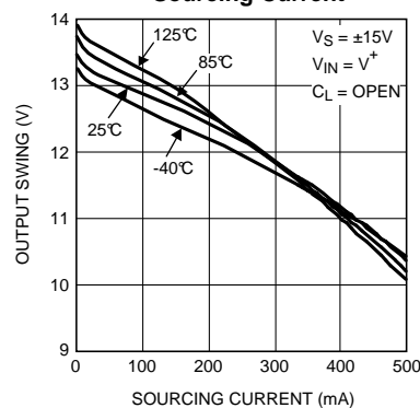
Positive Output Swing vs. Sourcing Current
