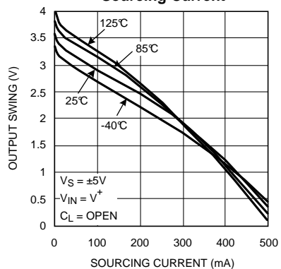
Positive Output Swing vs. Sourcing Current
