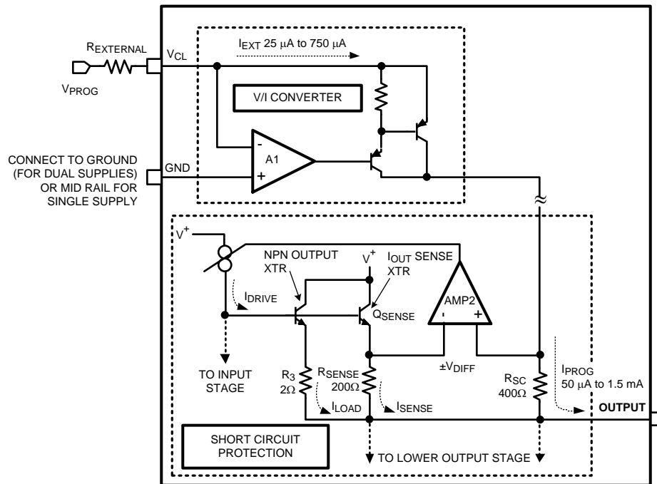
Figure 5. Simplified Diagram of Current Limit Control
