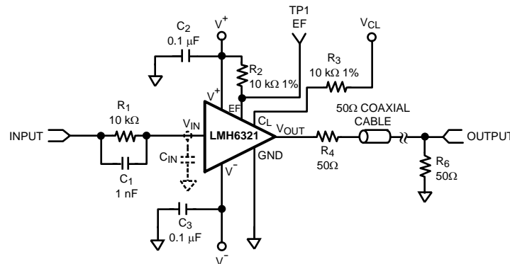
Figure 4. 50 \Omega Coaxial Cable Driver with Dual Supplies
