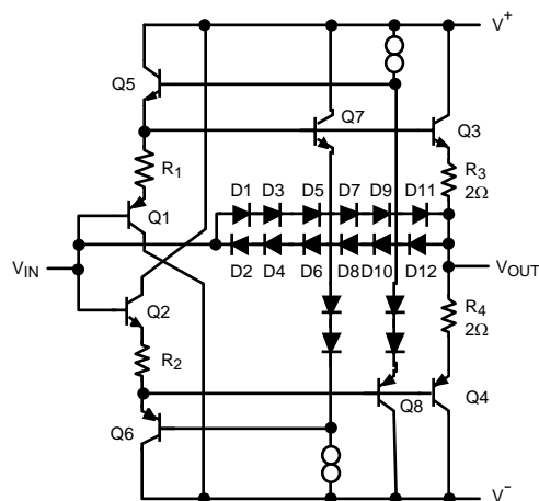
Figure 3. Simplified Schematic
