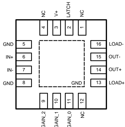
Figure 1. 16-Pin LLP (Top View)
