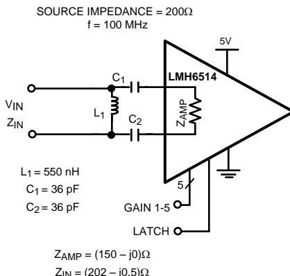
Figure 7. Differential 200Ω LC Conversion Circuit
