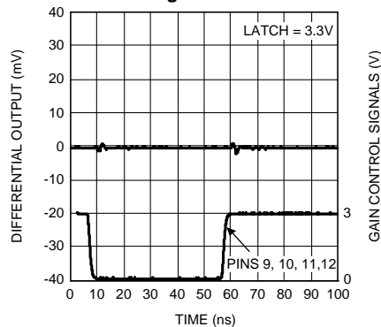
Digital Crosstalk
