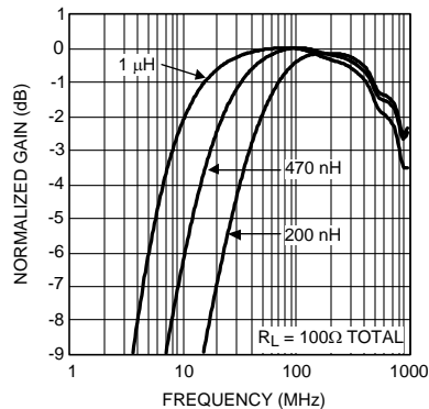
Figure 8. Bandwidth Changes Due to Different Inductor Values
