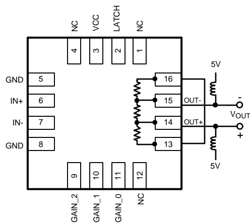
Figure 15. Alternate Connection for Low Gain Mode (200Ω Load)
