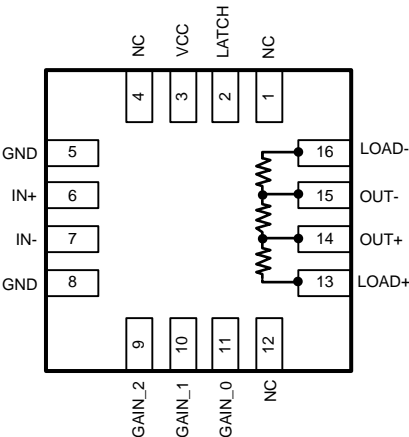
Figure 12. Internal Load Resistors
