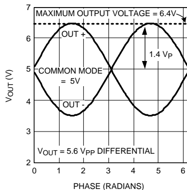
Figure 3. Output Voltage with Respect to the Output Common Mode
