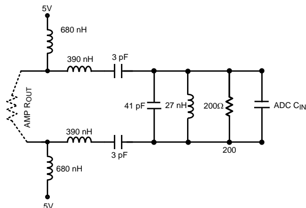
Figure 10. Bandpass Filter Center Frequency is 140 MHz with a 20 MHz Bandwidth Designed for 200 \Omega Impedance
