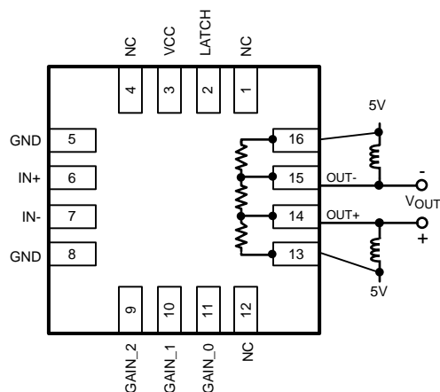
Figure 14. Using Low Gain Mode (200Ω Load)
