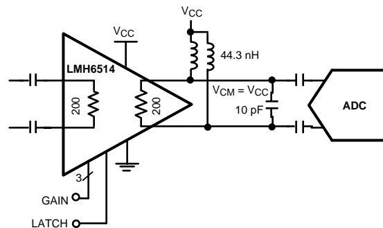
Figure 2. LMH6514 Typical Application
