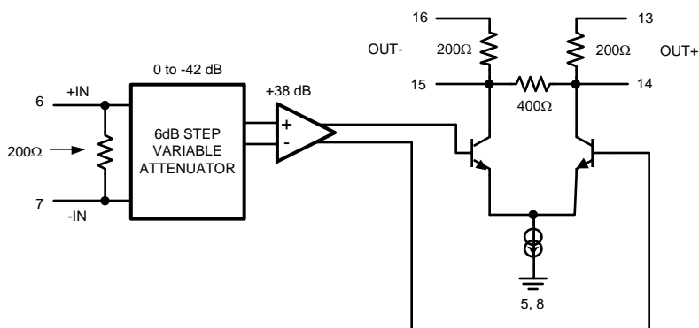
Figure 4. LMH6514 Block Diagram
