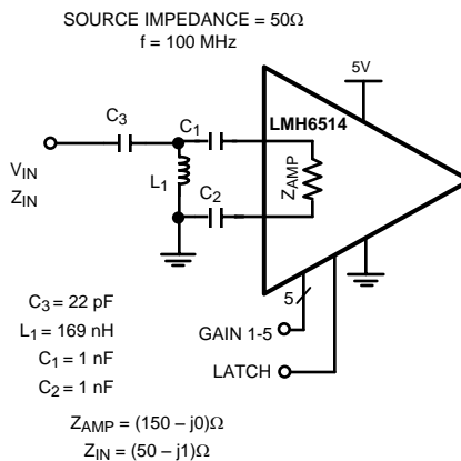
Figure 6. Single Ended Input with LC Matching
