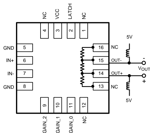
Figure 13. Using High Gain Mode (400Ω Load)
