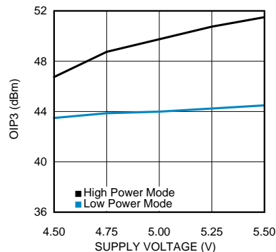
OIP3 vs Supply Voltage
