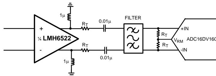
Figure 9. Output Configuration
