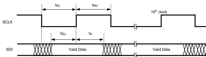
Figure 16. Write Timing Data Written to SDI Pin
