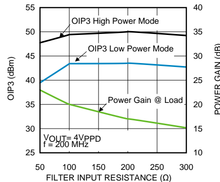
Figure 8. OIP3 and Power Gain vs Filter Impedance OIP3 and Gain Measured at Amplifier Output, Filter Back Terminated
