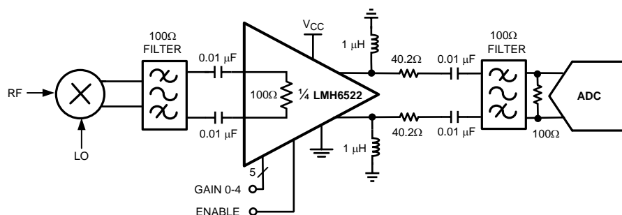
Figure 3. LMH6522 Typical Application
