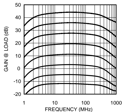
Figure 11. Frequency Response of Cascaded Amplifiers
