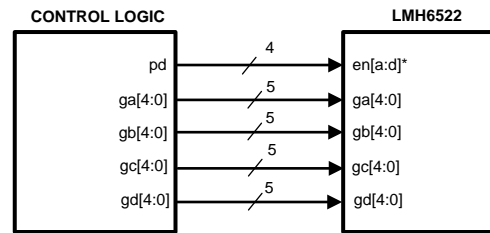
Figure 12. Parallel Mode Connection
