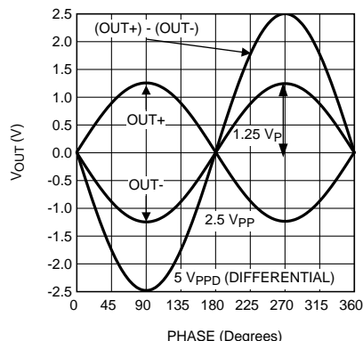
Figure 7. Differential Output Voltage
