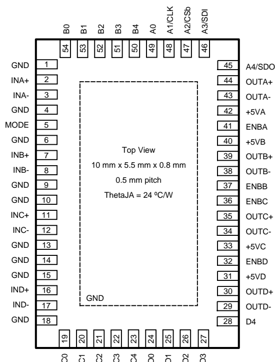
Figure 2. 54-Pin LLP - Top View
