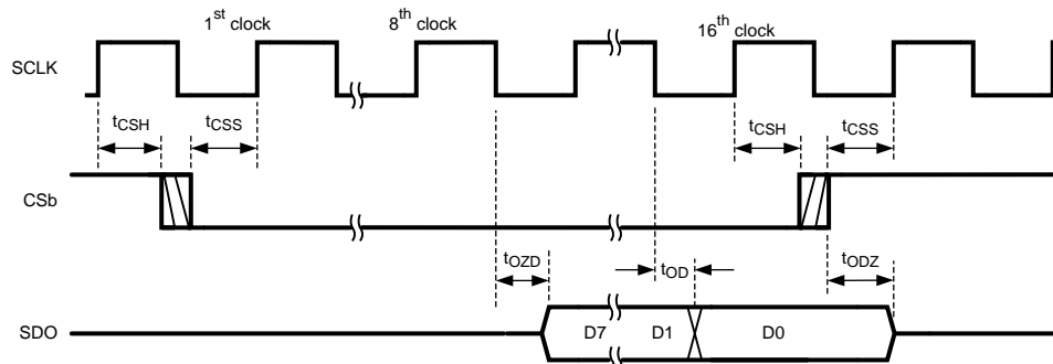
Figure 15. Read Timing
