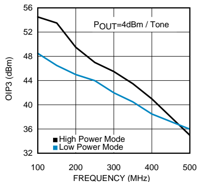
OIP3 vs Frequency
