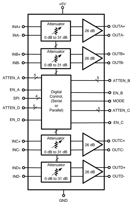
Figure 4. LMH6522 Block Diagram
