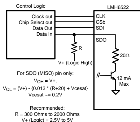
Figure 14. Internal Operation of the SDO pin
