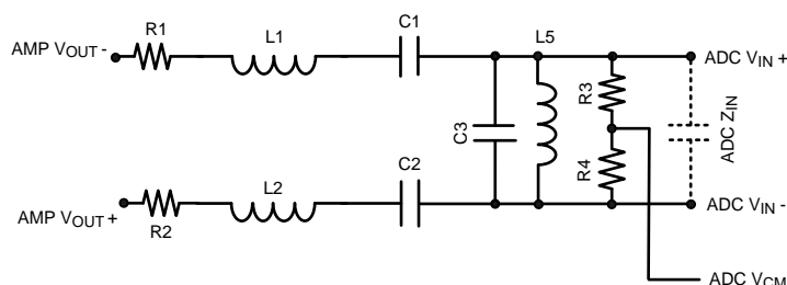
Figure 17. Sample Filter
