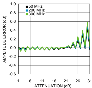
Gain Step Amplitude Error
