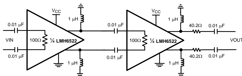
Figure 10. Schematic for Cascaded Amplifiers
