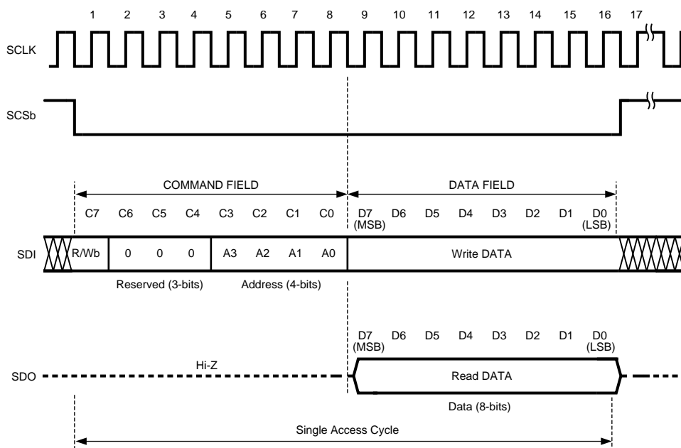
Figure 13. Serial Interface Protocol (SPI compatible)
