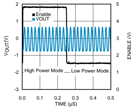
Figure 18. Signal Output During Mode Change from High Power Mode to Low Power Mode
