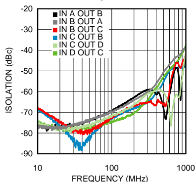
Isolation, Adjacent Channels
