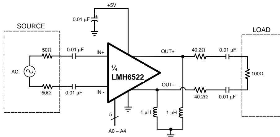
Figure 5. LMH6522 Basic Connections Schematic
