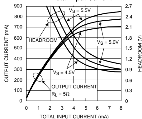
Headroom & Output Current vs. Total Input Current
