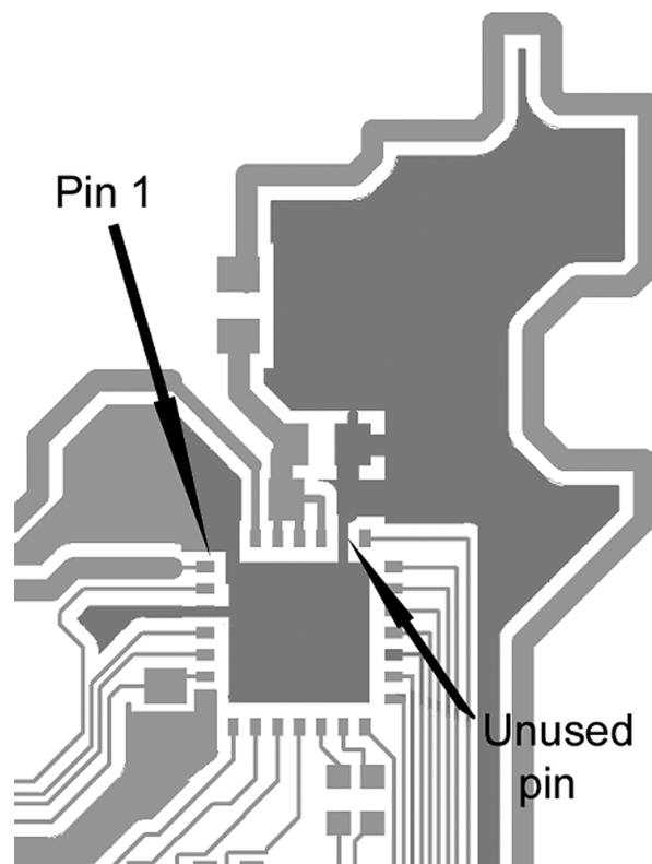
Figure 12. Heat Sinking
