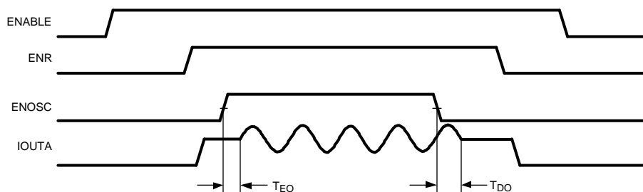
Figure 7. Oscillator Timing
