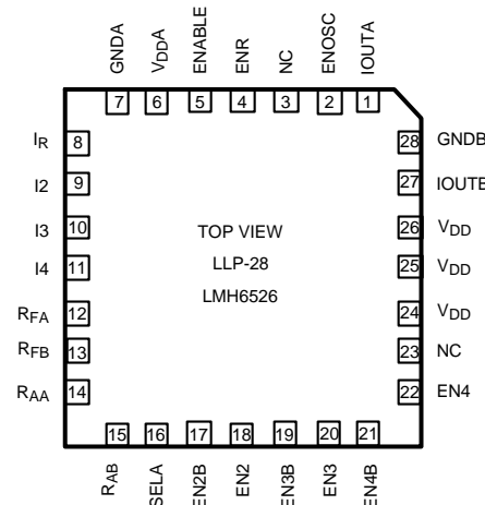
Figure 2. Top View
