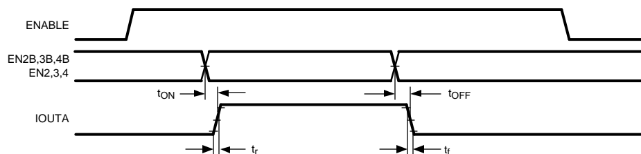
Figure 6. Write Timing
