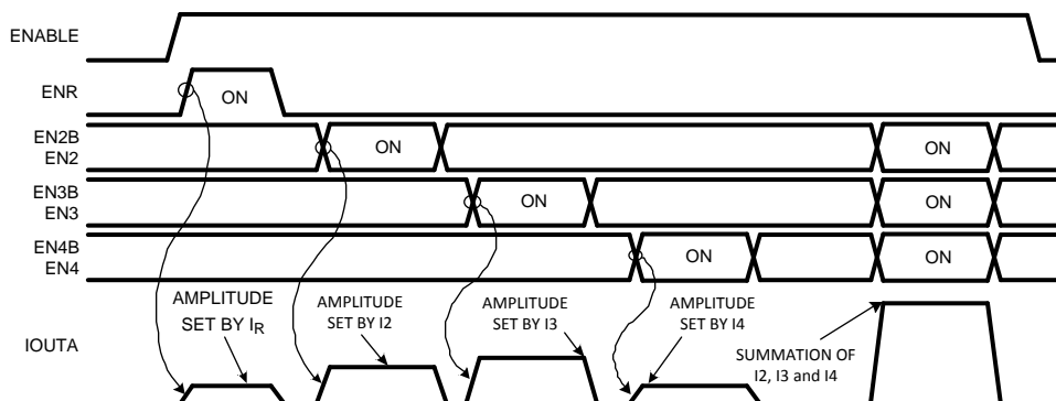
Figure 3. Functional Timing Diagram
