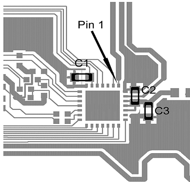
Figure 11. Decoupling Capacitors
