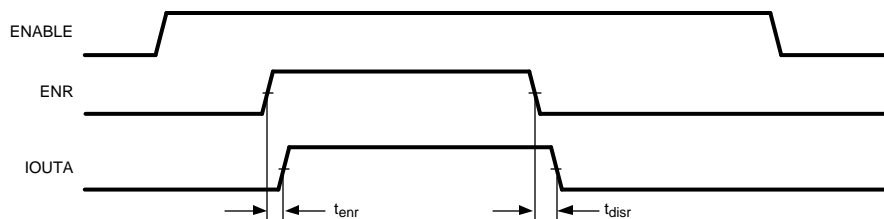
Figure 5. Read Timing
