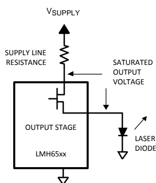
Figure 8. Output Configuration
