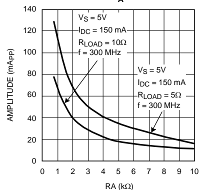
Oscillator Amplitude vs. R_A
