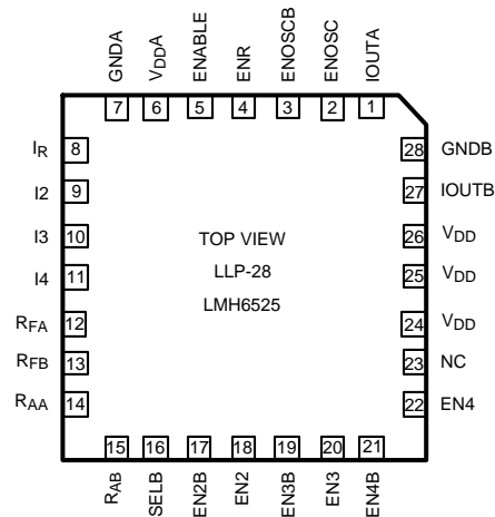
Figure 1. Top View
