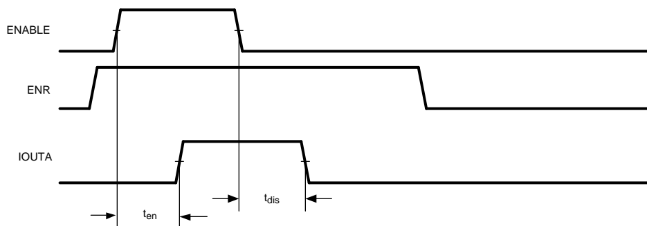
Figure 4. Enable Timing
