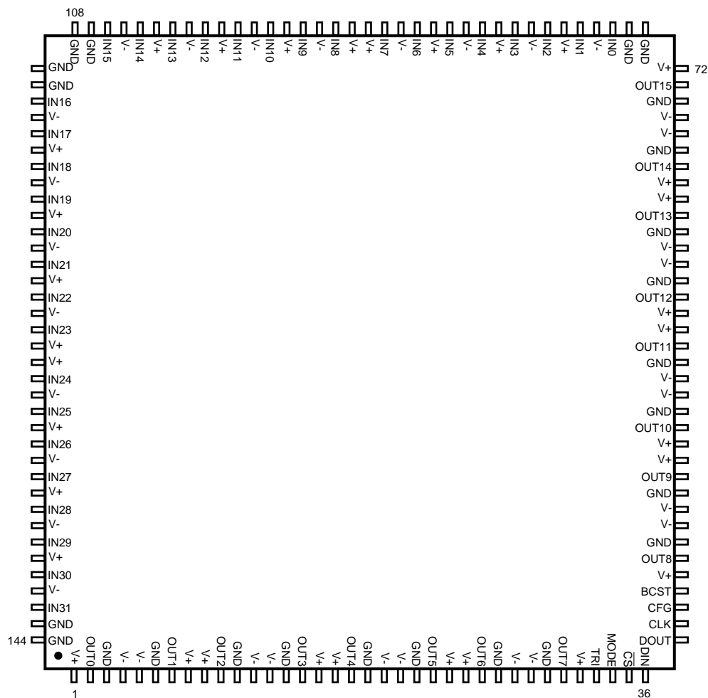
Figure 1. Top View
