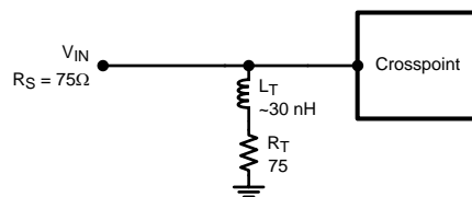
Figure 8. Use of Termination Inductor to Increase Bandwidth
