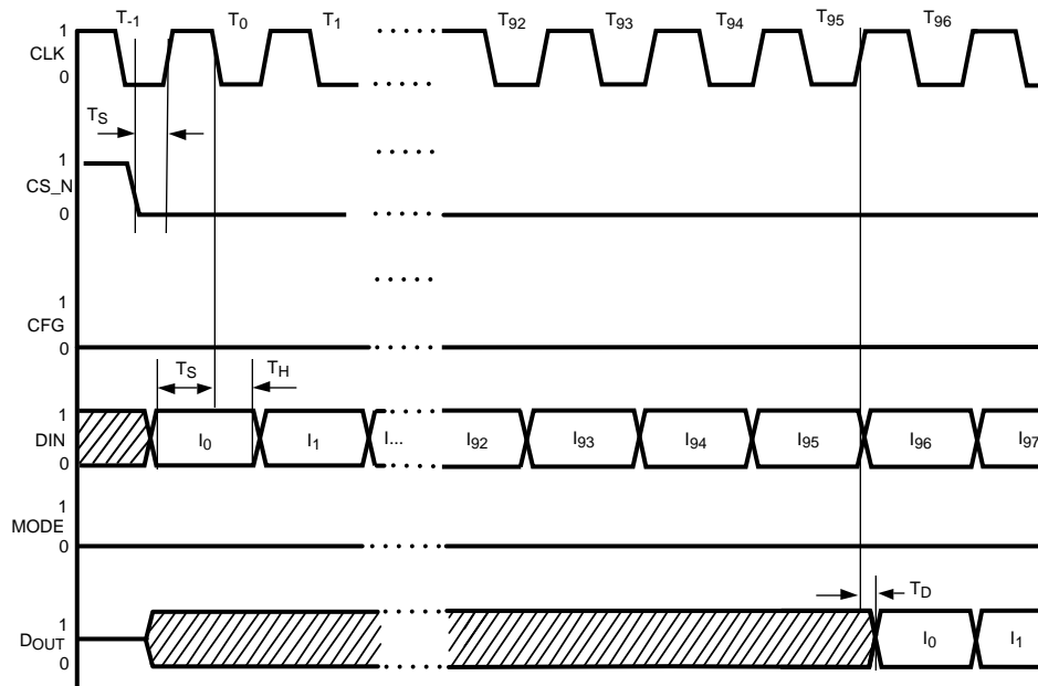
Figure 17. Timing Diagram for Daisy Chain Operation
