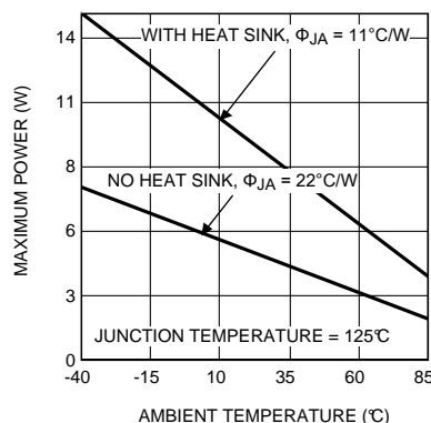
Figure 18. Maximum Dissipation vs. Ambient Temperature
