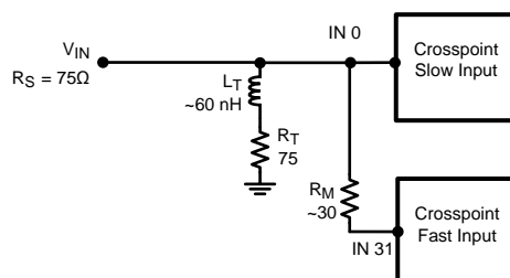
Figure 10. Inductor Termination with Mismatched Channels
