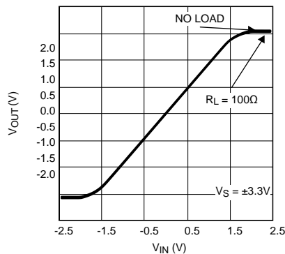
Output Swing
