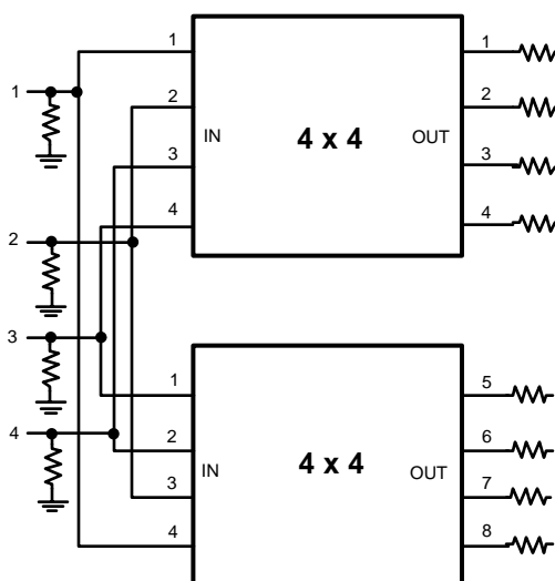
Figure 4. Output Expansion no Buffers (Only 4 input and 4 output channels shown for illustration purposes.)
