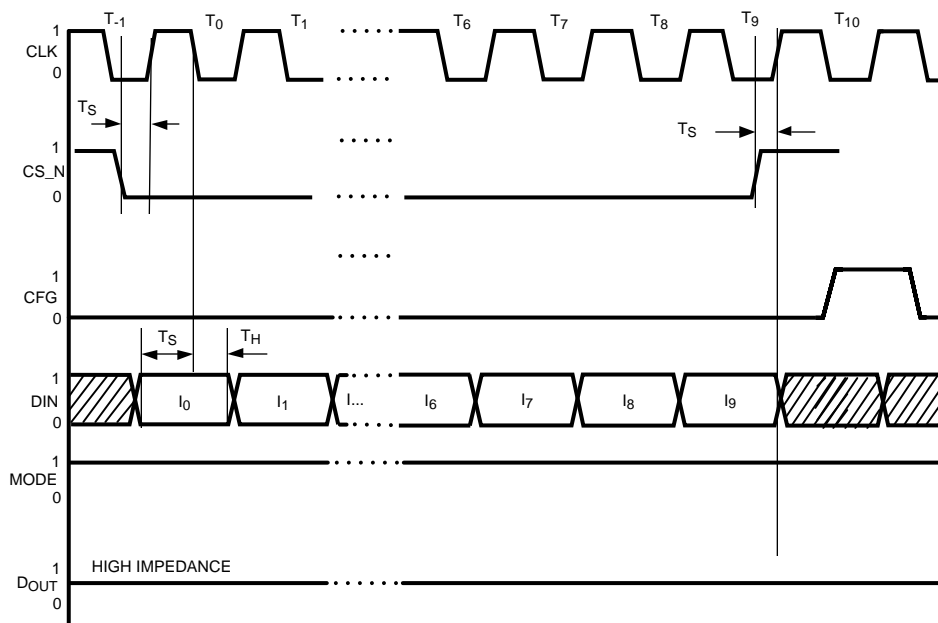
Figure 16. Timing Diagram for Addressed Mode
