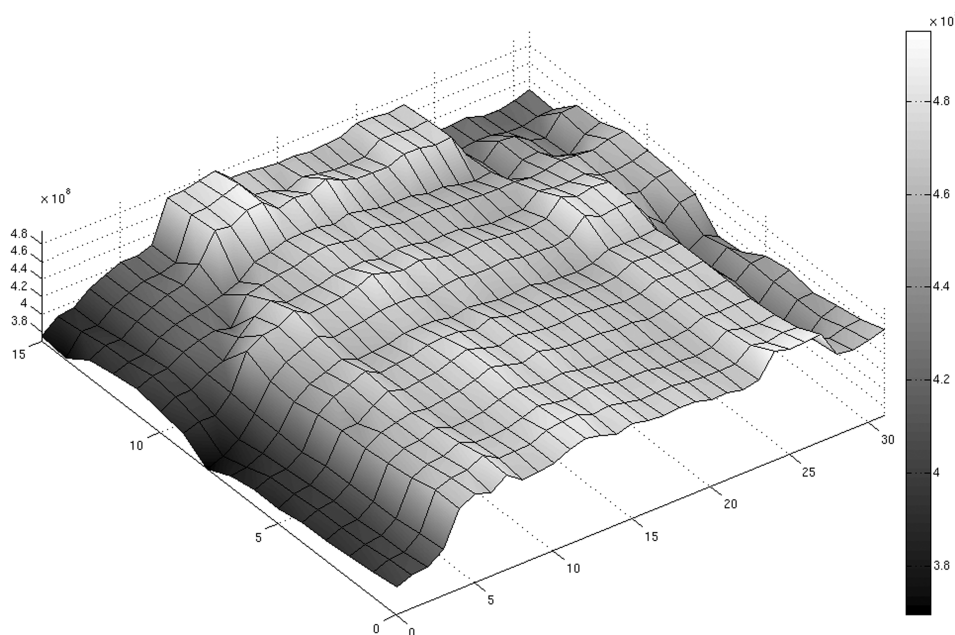
Figure 7. Bandwidth Variation over Channel Combinations
