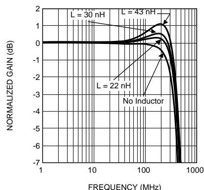
Figure 9. Termination Inductor Bandwidth Enhancement Using Input 0
