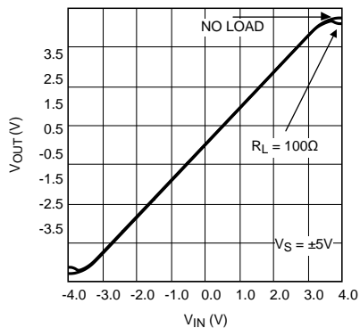
Output Swing
