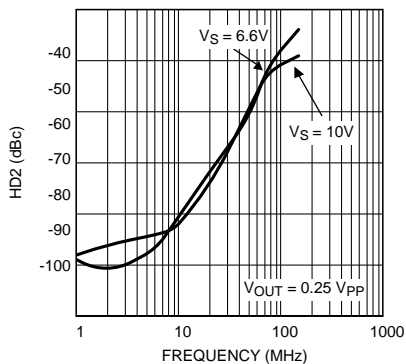
Second Order Distortion
