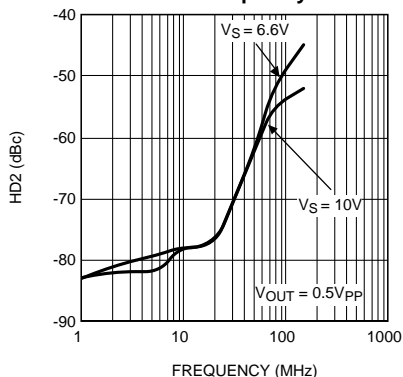
Second Order Distortion (HD2)
