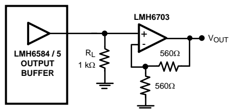
Figure 13. Buffered Output
