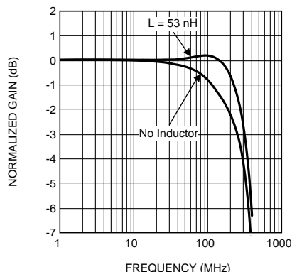
Figure 12. Termination Inductor Bandwidth Enhancement Using Input 0 Two LMH6585s Connected for Output Expansion
