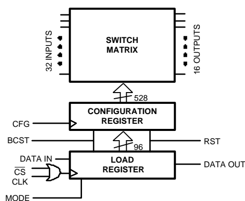
Figure 14. Block Diagram
