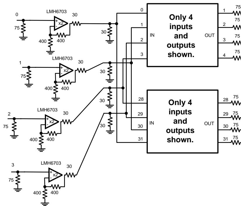
Figure 2. Output Expansion with Buffers
