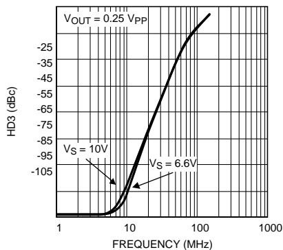
Third Order Distortion
