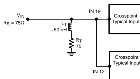
Figure 11. Inductor Termination with Matched Channels
