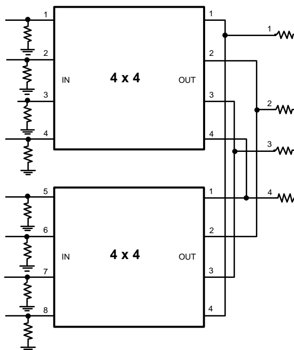
Figure 5. Input Expansion with Shared Termination Resistors (Only 4 input and 4 output channels shown for illustration purposes.)
