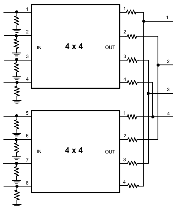
Figure 6. Input Expansion with Separate Termination Resistors (Only 4 input and 4 output channels shown for illustration purposes.)
