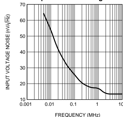
Input Referred Voltage Noise
