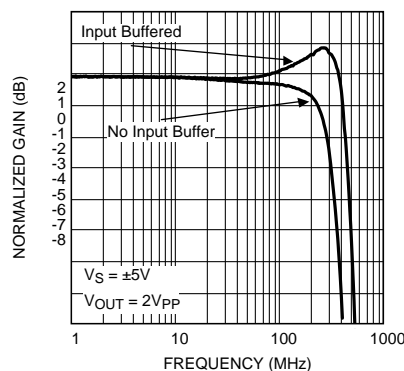
Figure 3. Frequency Response for Buffered and Unbuffered Output expansion
