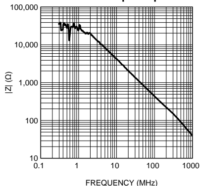
Disabled Output Impedance
