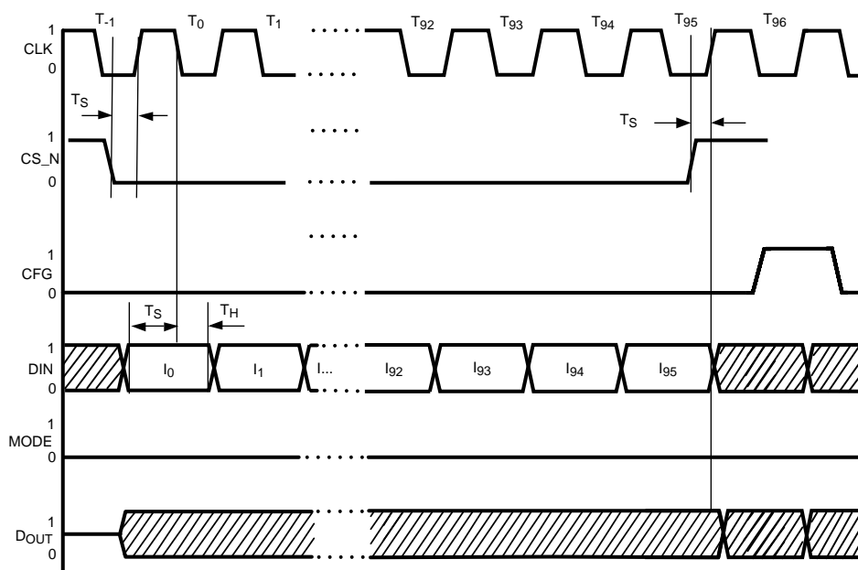
Figure 15. Timing Diagram for Serial Mode
