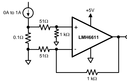
Figure 13. Current Sense Amplifier
