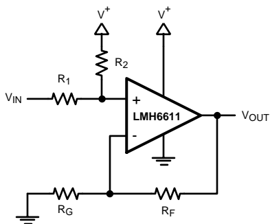
Figure 11. DC Level Shifting
