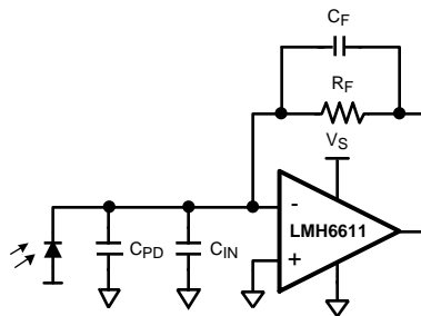
Figure 14. Photodiode Modeled with Capacitance Elements
