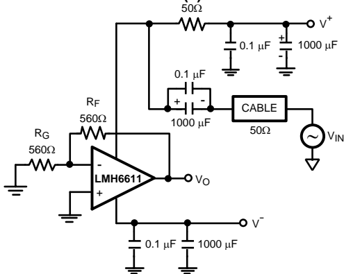
Circuit for Positive (+) PSRR Measurement
