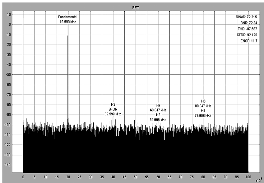
Figure 10. The FFT Plot of Differential to Differential ADC Driver
