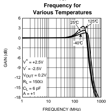
Closed Loop Gain vs. Frequency for Various Temperatures
