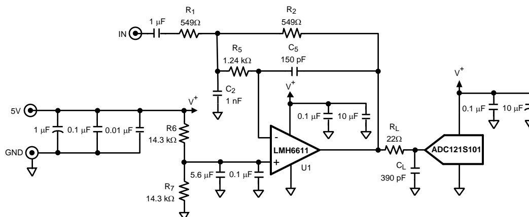
Figure 6. Single to Single ADC Driver
