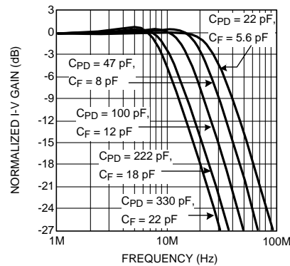
Figure 16. Frequency Response for Various Photodiode and Feedback Capacitors
