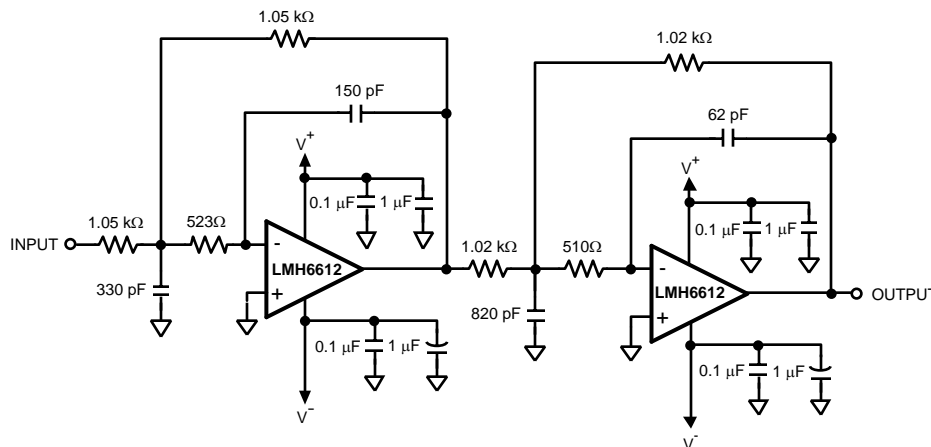
Figure 12. 4 th Order Multiple Feedback Low-Pass Filter
