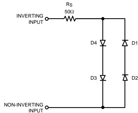
Figure 4. Input Equivalent Circuit During Shutdown
