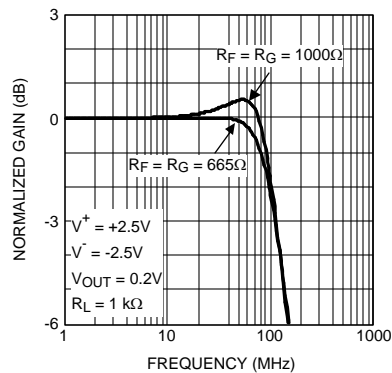
Figure 5. Closed Loop Gain vs. Frequency and R_F = R_G
