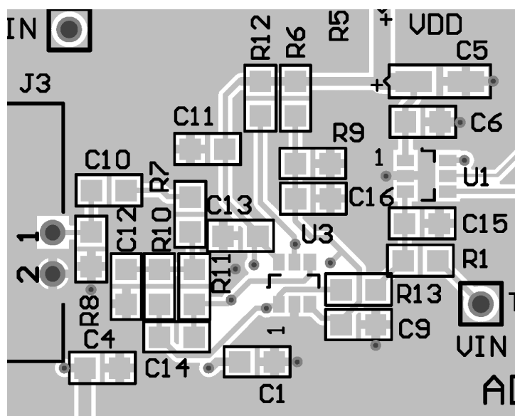
Figure 7. LMH6611 and ADC121S101 Layout
