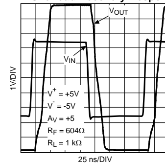
Overload Recovery Response
