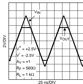
Figure 3. Input and Output Shown with CMVR Exceeded
