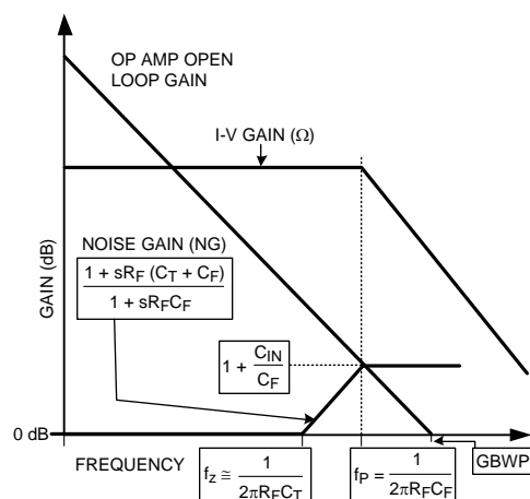
Figure 15. Bode Plot of Noise Gain Intersecting with Op Amp Open Loop Gain
