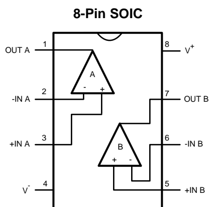
Figure 2. Top View
