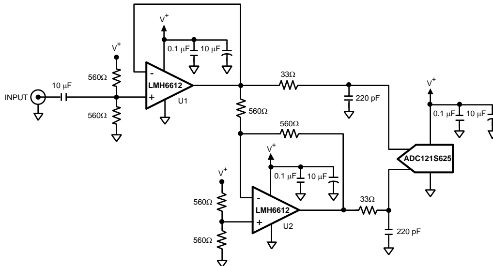
Figure 8. Single-Ended to Differential ADC Driver
