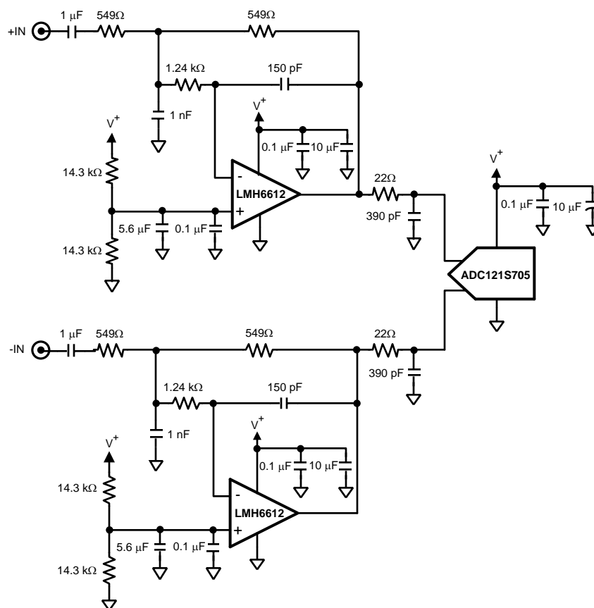
Figure 9. Differential to Differential ADC Driver
