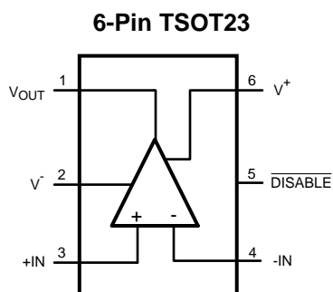
Figure 1. Top View
