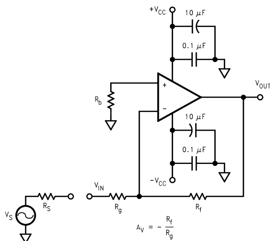
Figure 7. Inverting Amplifier Configuration
