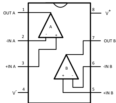
Figure 3. 8-Pin SOIC and MSOP (LMH6655) Top View
