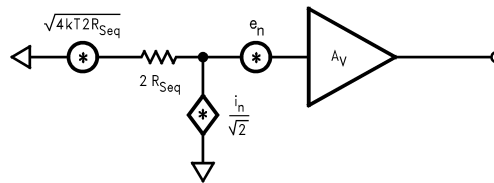
Figure 9. Noise Model with R_f \parallel R_g = R_{seq}
