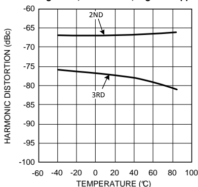
Harmonic Distortion vs. Temperature
