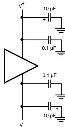
Figure 4. Supply Bypass Capacitors
