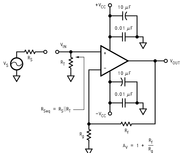
Figure 6. Non-Inverting Amplifier Configuration
