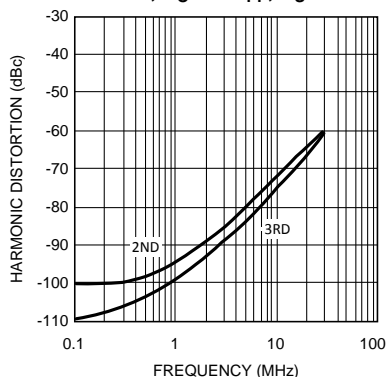
Harmonic Distortion vs. Frequency
