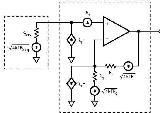
Figure 8. Non-Inverting Amplifier Noise Model
