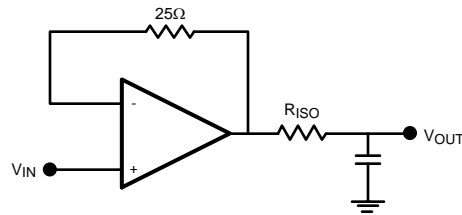
Figure 5. Isolation Resistor Placement
