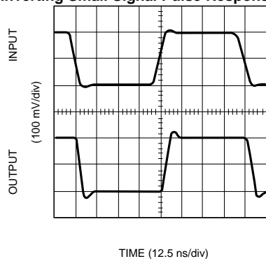
Non-Inverting Small Signal Pulse Response ( V_S = \pm 5\text{V} )
