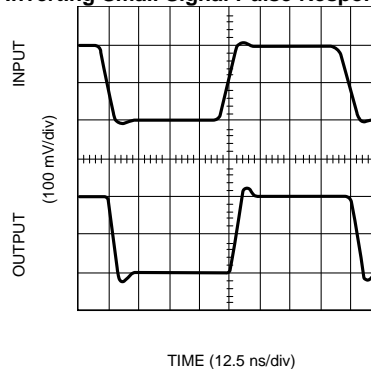
Inverting Small Signal Pulse Response ( V_S = 5\text{V} )
