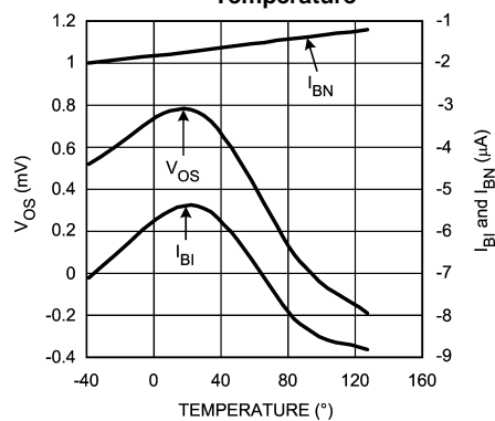
Temperature
