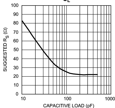
Suggested R_S vs. C_L
