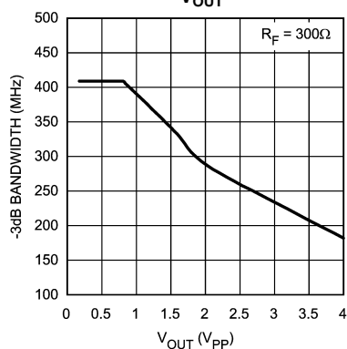
-3dB Bandwidth
