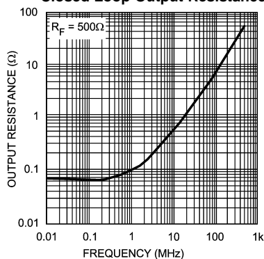
Closed Loop Output Resistance
