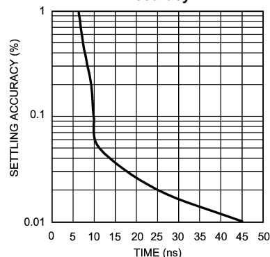
DC Errors
