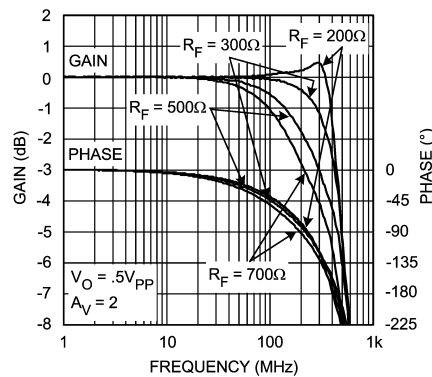
Figure 4. Frequency Response vs. R_F
