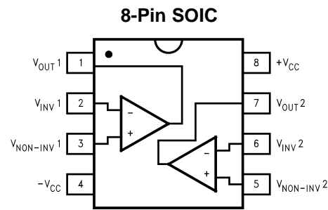
Figure 1. Top View
