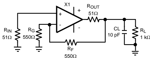
Figure 7. Series Output Resistor Inside Feedback Loop
