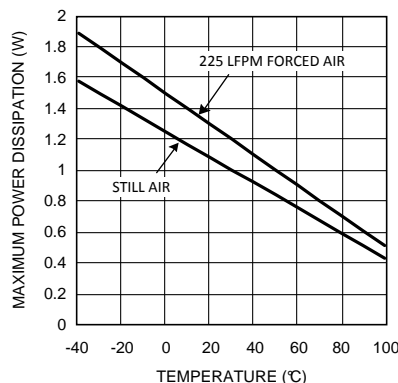
Figure 8. Maximum Power Dissipation
