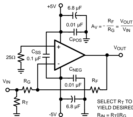
Figure 3. Recommended Inverting Gain Circuit
