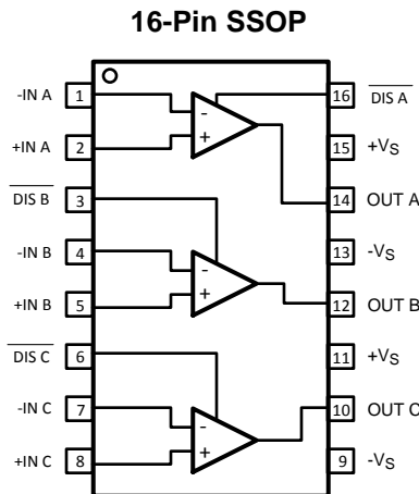
Figure 1. Top View
