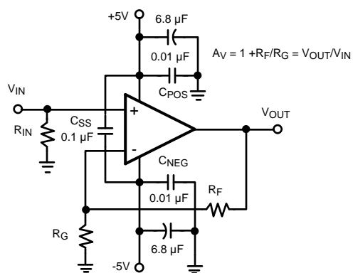
Figure 2. Recommended Non-Inverting Gain Circuit
