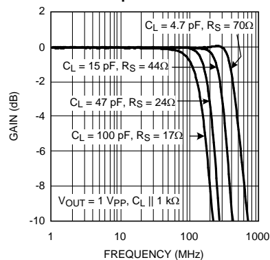
Frequency Response vs. Capacitive Load
