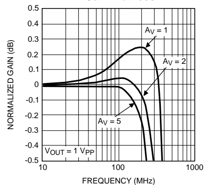
Gain Flatness
