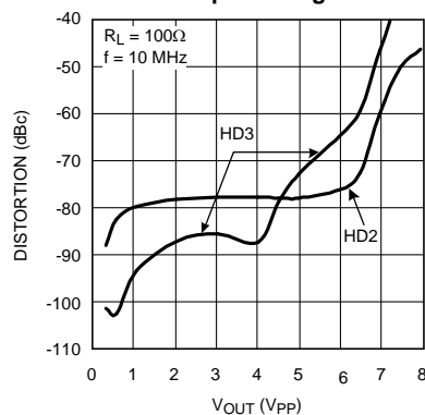
Distortion vs. Output Voltage
