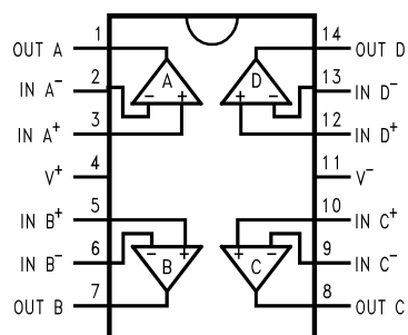
Figure 2. 14-Pin TSSOP/SOIC
