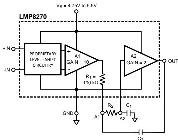
Figure 11. Low-Pass Filter With LMP8270
