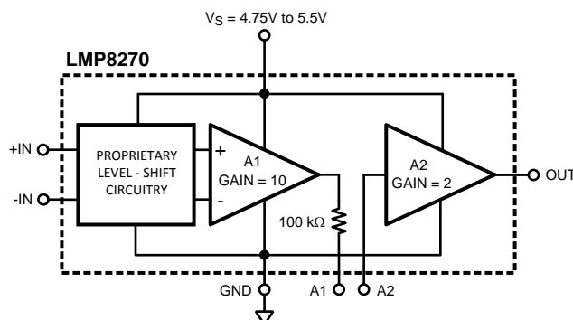
Figure 3. LMP8270
