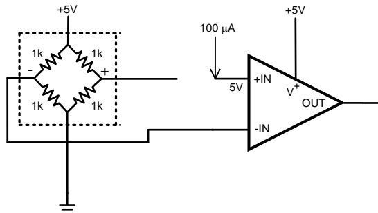
Figure 56. Open Input
