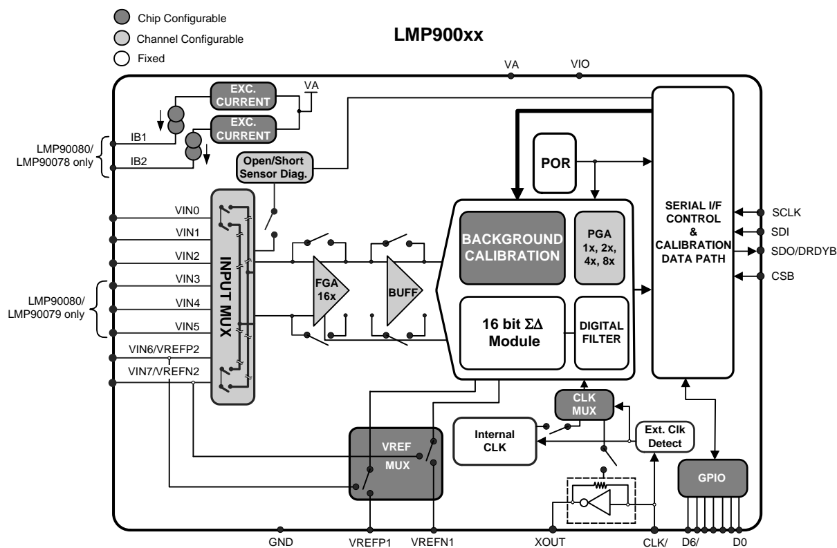
Figure 1. Block Diagram
