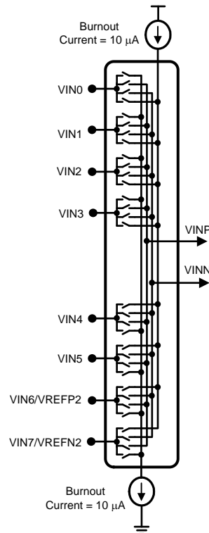
Figure 44. Burnout Currents
