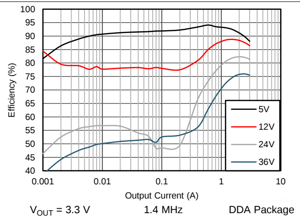
Figure 28. Efficiency
