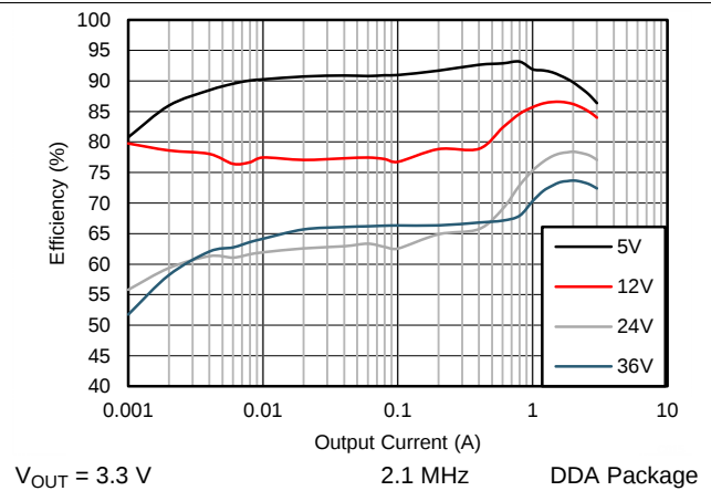
Figure 30. Efficiency
