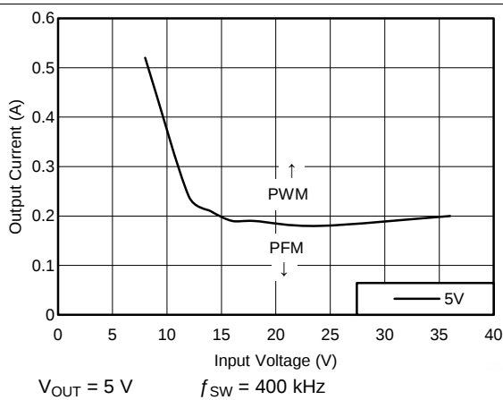
Figure 39. Mode Change Thresholds
