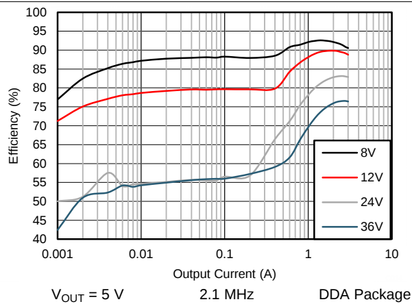
Figure 29. Efficiency
