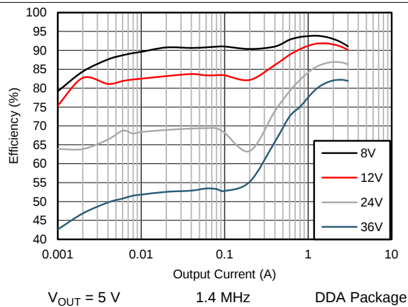
Figure 27. Efficiency
