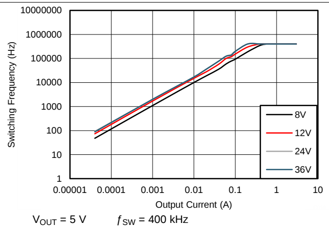
Figure 40. Switching Frequency vs Output Current
