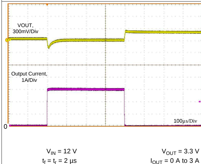
Figure 47. Load Transient
