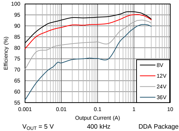
Figure 25. Efficiency
