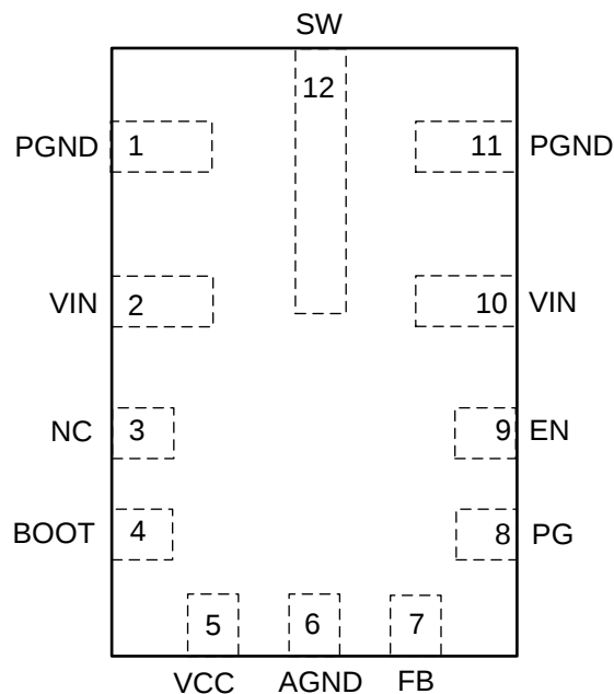
RNX Package 12-Pin VQFN Top View
