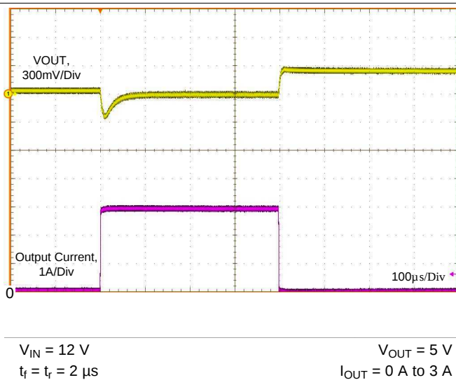
Figure 41. Load Transient
