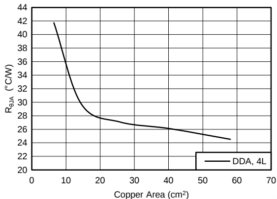
Figure 22. Typical R_{\theta JA} vs Copper Area for a Four-Layer Board and the HSOIC (DDA) Package
