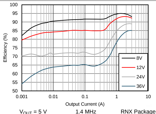
Figure 33. Efficiency
