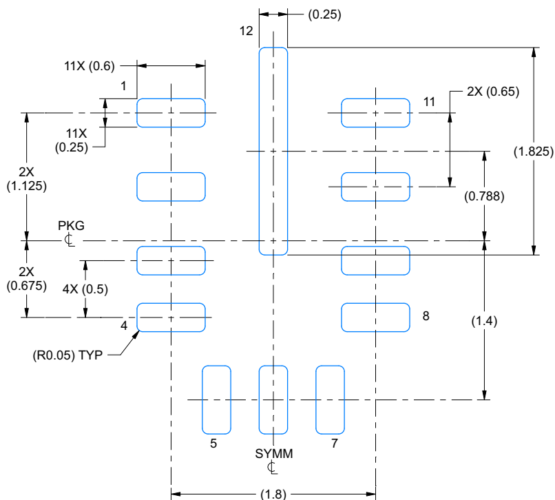
LAND PATTERN EXAMPLE EXPOSED METAL SHOWN SCALE:25X
