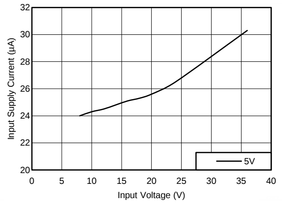
Figure 38. Input Supply Current
