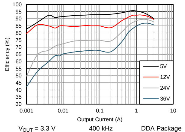
Figure 26. Efficiency
