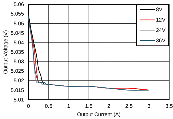
Figure 37. Line and Load Regulation
