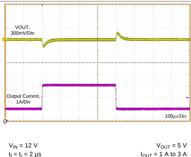
Figure 42. Load Transient
