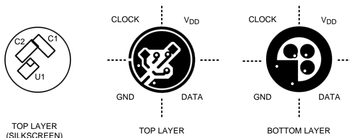
Figure 12. PCB Layout
