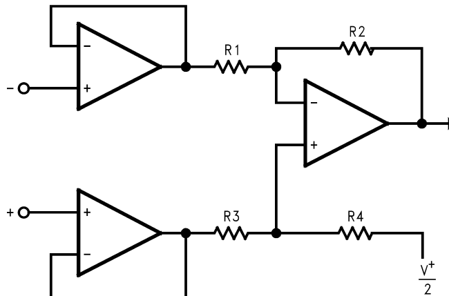
Figure 11. Three-Op-Amp Instrumentation Amplifier
