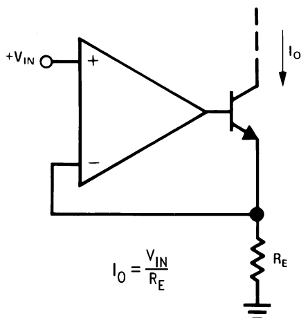
Figure 24. High Compliance Current Sink
