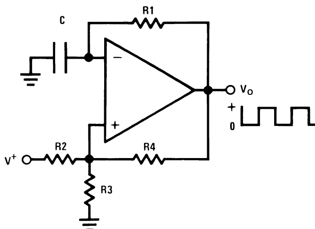
Figure 22. Squarewave Generator
