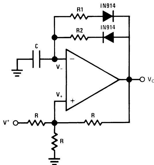
Figure 19. Pulse Generator
