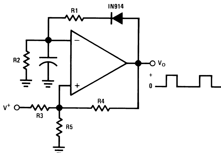
Figure 21. Pulse Generator
