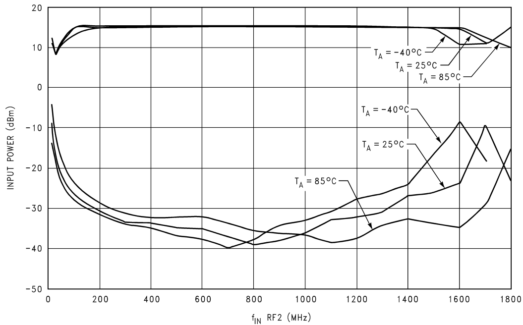
LMX2335U and LMX2336U f_{IN} RF2 Input Power Vs Frequency V_{CC} = V_P RF2 = 5.5V
