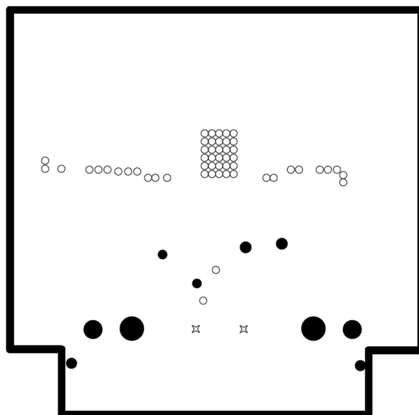
Figure 18. Internal Layer 1 (Ground)
