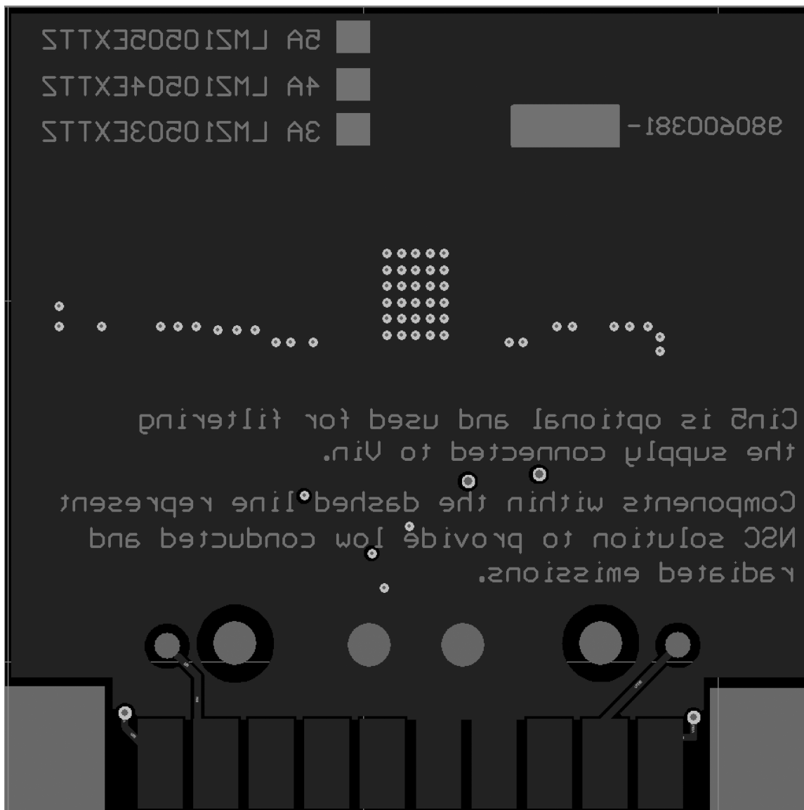
Figure 20. Bottom Copper
