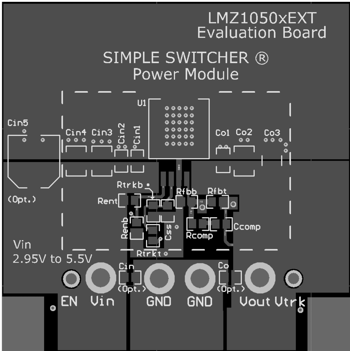
Figure 17. Top Copper
