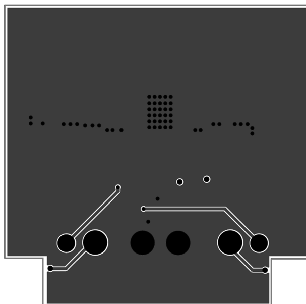
Figure 19. Internal Layer 2 (Ground and Signal Traces)
