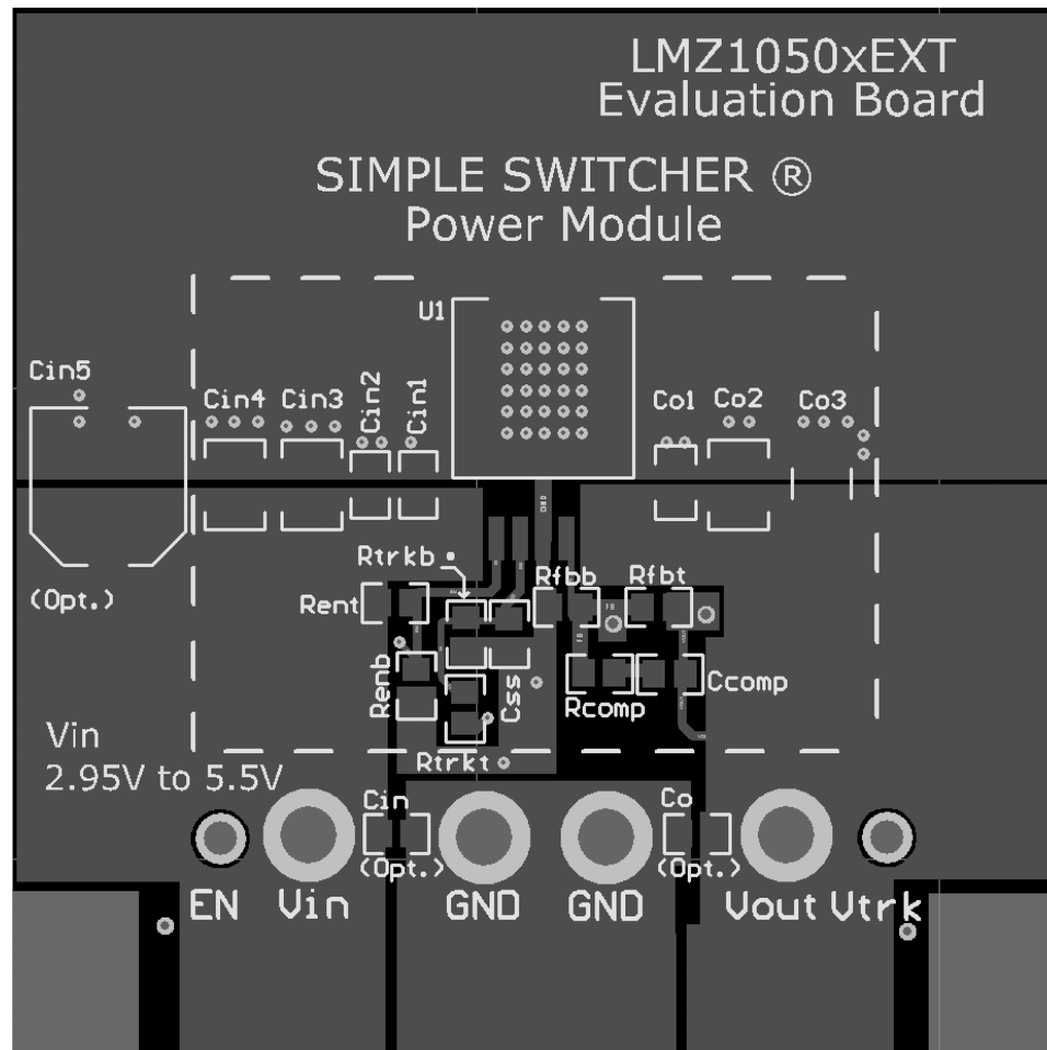
Figure 20. Top Copper
