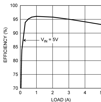
Efficiency ( V_{OUT} = 3.3V )
