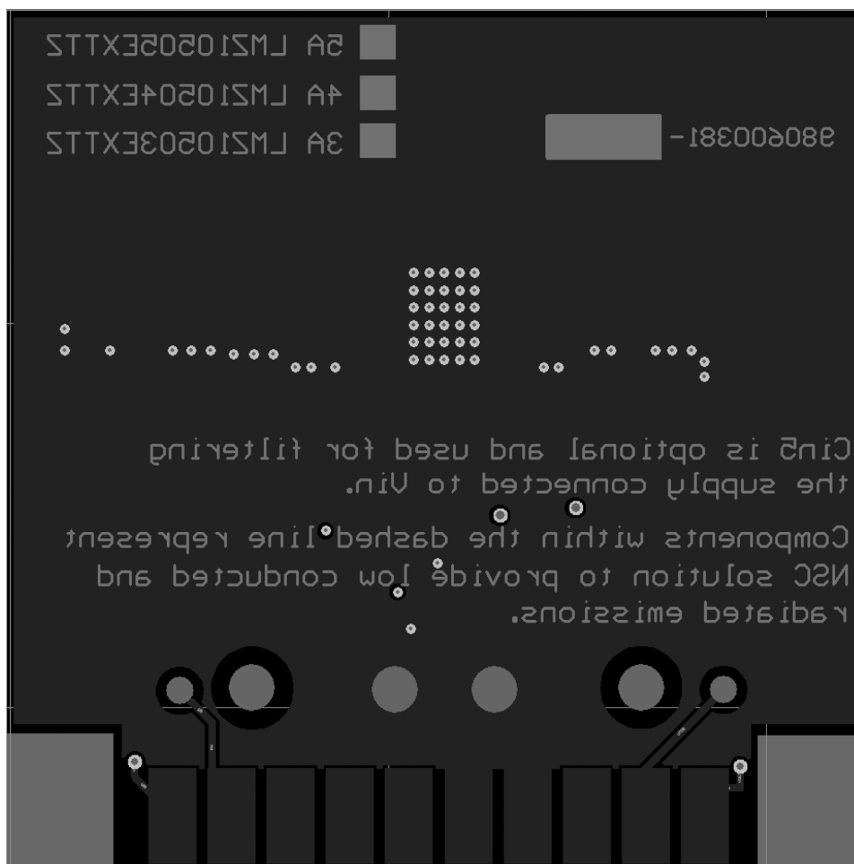
Figure 23. Bottom Copper
