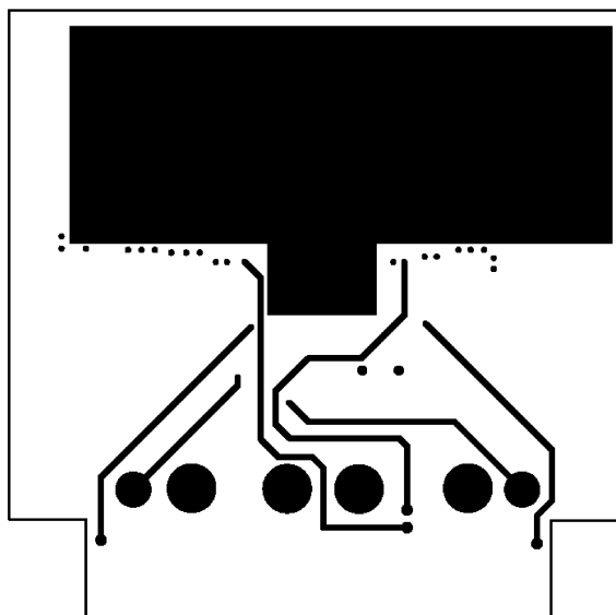
Figure 22. Internal Layer 2 (Ground and Signal Traces)
