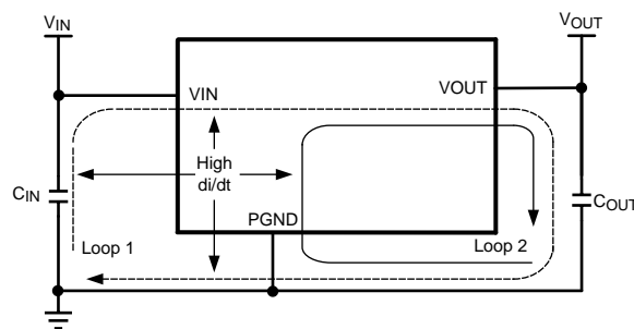
Figure 8. High Current Loops
