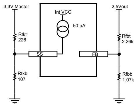
Figure 7. Tracking option input detail
