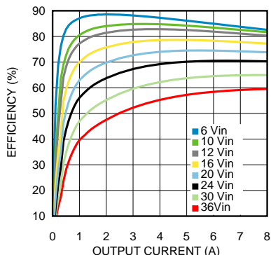
Efficiency 1.5V output @ 85°C
