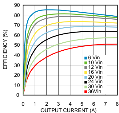
Efficiency 1.2V output @ 25°C
