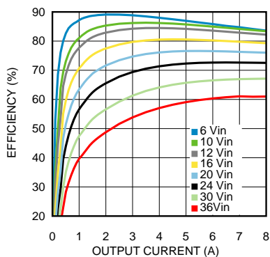
Efficiency 1.5V output @ 25°C
