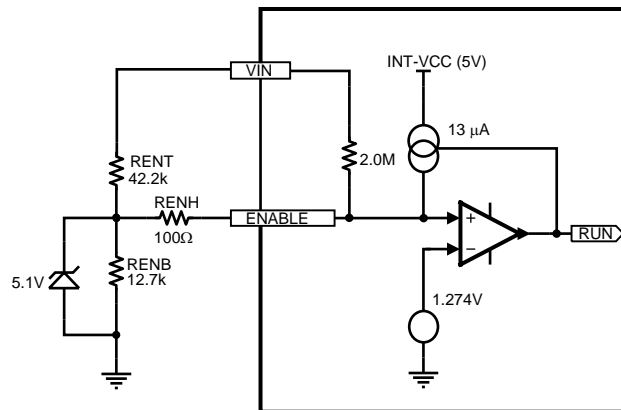
Figure 6. Enable input detail
