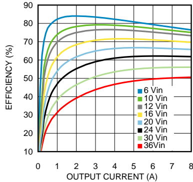
Efficiency 1.0V output @ 85°C
