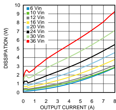
Dissipation 1.5V output @ 25°C
