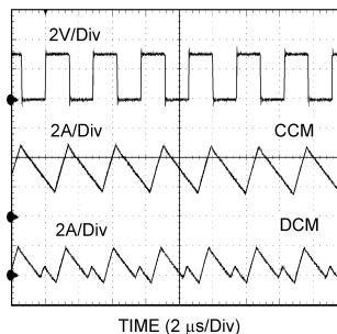
Figure 10. CCM and DCM Operating Modes V_{IN} = 12\text{V} , V_O = 3.3\text{V} , I_O = 3\text{A}/0.3\text{A}
