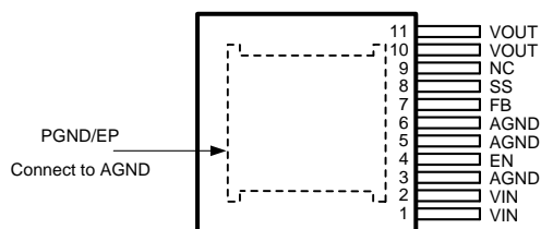
Figure 5. Top View - 11-Lead TO-PMOD
