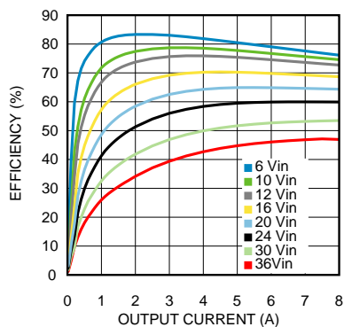
Efficiency 5.0V output @ 85°C
