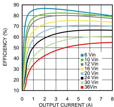
Efficiency 1.5V output @ 85°C
