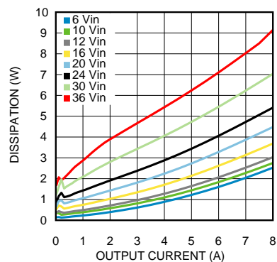
Dissipation 5.0V output @ 85°C
