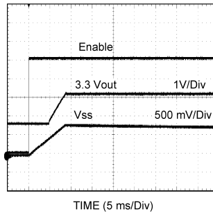
Figure 9. Pre-Biased Startup
