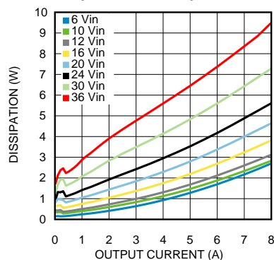
Dissipation 1.2V output @ 25°C
