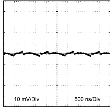
Output ripple 12V_{IN} 3.3V_O @ 5A, BW = 20 MHz
