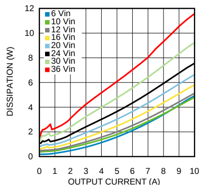
Dissipation 3.3V output @ 85°C
