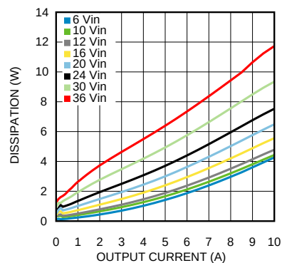
Dissipation 1.0V output @ 85°C
