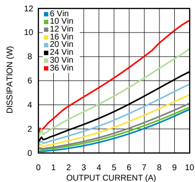
Dissipation 5.0V output @ 85°C
