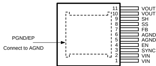
Figure 4. Top View 11-Lead TO-PMOD
