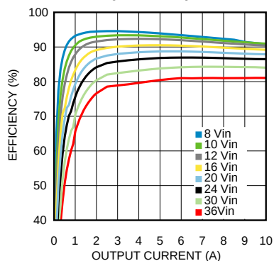
Efficiency 3.3V output @ 85°C
