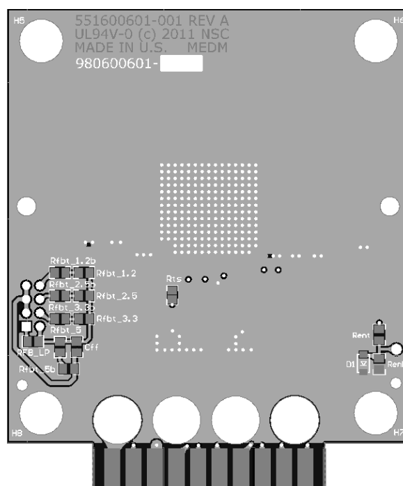
Figure 14. Layout example
