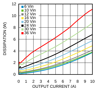
Dissipation 1.2V output @ 25°C
