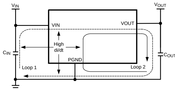
Figure 7. High Current Loops
