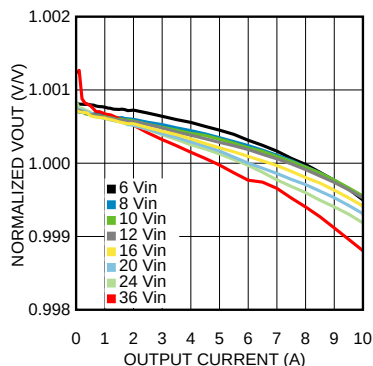
Normalized line and load regulation V_{OUT} = 3.3V
