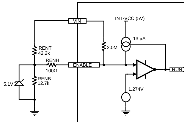
Figure 5. Enable input detail
