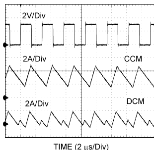
Figure 12. CCM and DCM Operating Modes V_{IN} = 12V , V_O = 3.3V , I_O = 3A/0.3A
