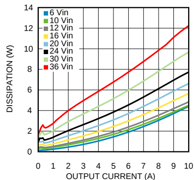
Dissipation 1.5V output @ 85°C
