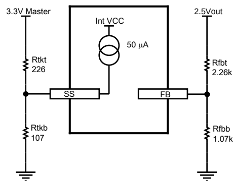
Figure 6. Tracking option input detail
