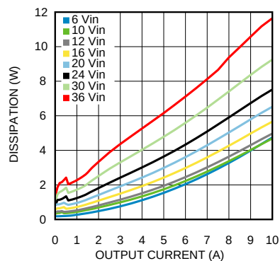
Dissipation 1.8V output @ 85°C
