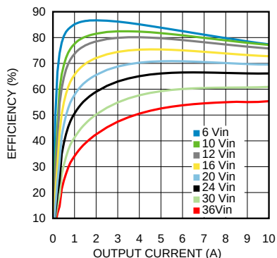
Efficiency 1.5V output @ 85°C
