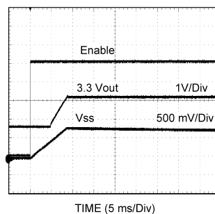
Figure 11. Pre-Biased Startup
