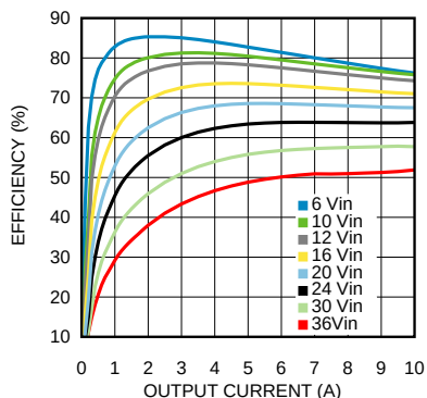
Efficiency 1.2V output @ 25°C
