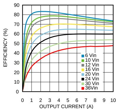
Efficiency 5.0V output @ 85°C
