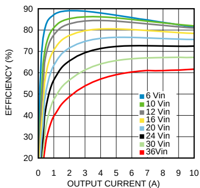
Efficiency 1.5V output @ 25°C
