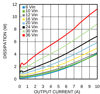
Dissipation 1.5V output @ 25°C
