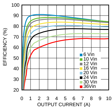
Efficiency 1.8V output @ 85°C
