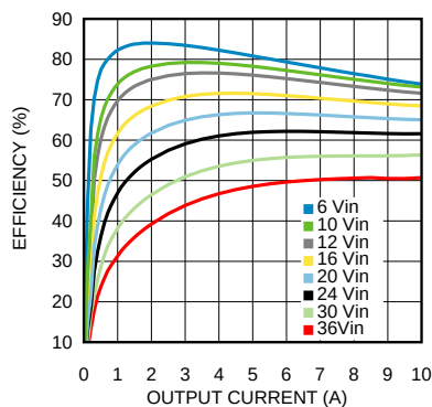
Efficiency 1.0V output @ 85°C
