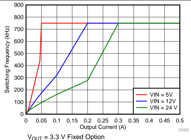
Figure 20. Auto PFM Mode Switching Frequency vs Output Current
