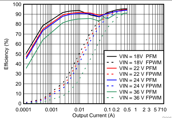
Figure 51. Efficiency
