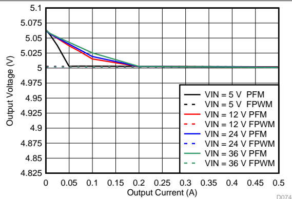
Figure 65. Line and Load Regulation for V_{OUT} = 5\text{ V}
