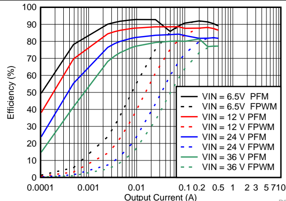
Figure 39. Efficiency
