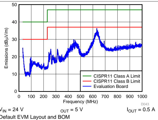
Figure 6. Radiated EMI
