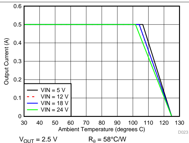
Figure 12. Ambient Temperature vs Output Current
