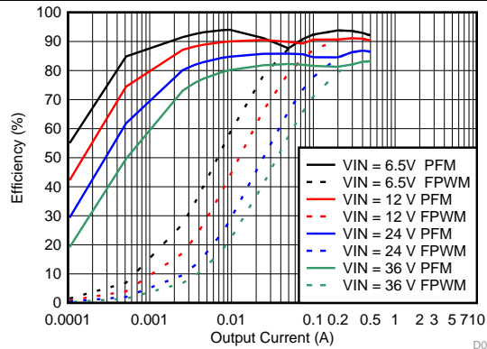
Figure 33. Efficiency
