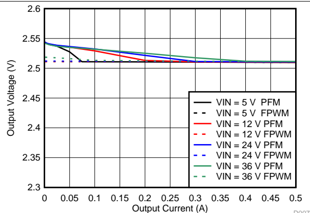
Figure 61. Line and Load Regulation
