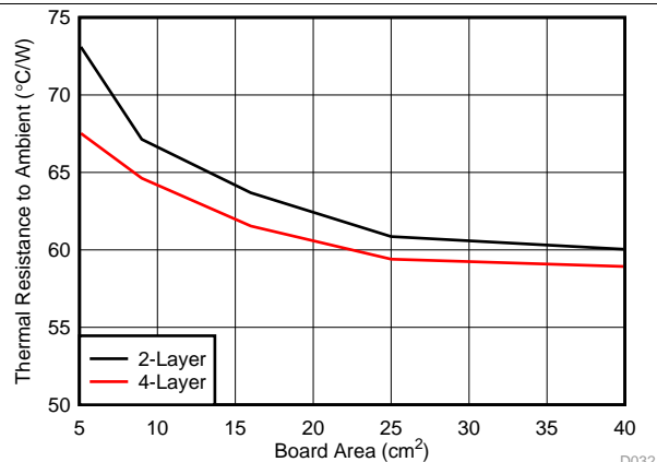
Figure 7. Package Thermal Resistance vs Board Copper Area, No Air Flow
