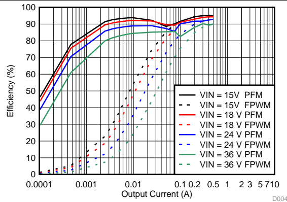
Figure 45. Efficiency
