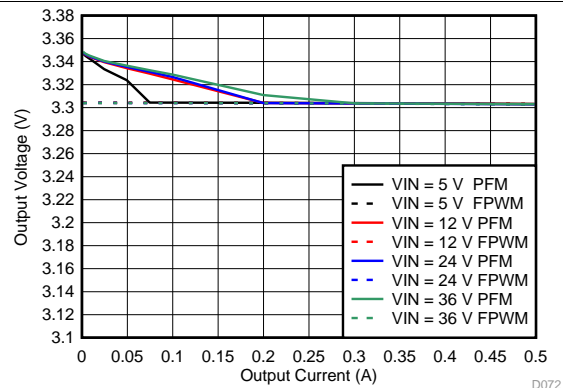
Figure 66. Line and Load Regulation for V_{OUT} = 3.3\text{ V}
