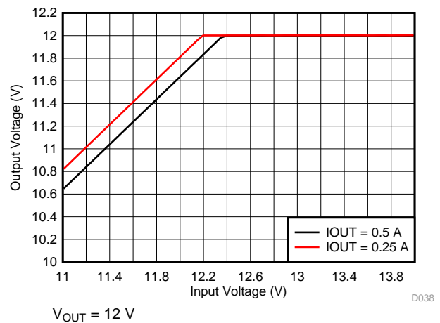
Figure 4. Dropout Voltage
