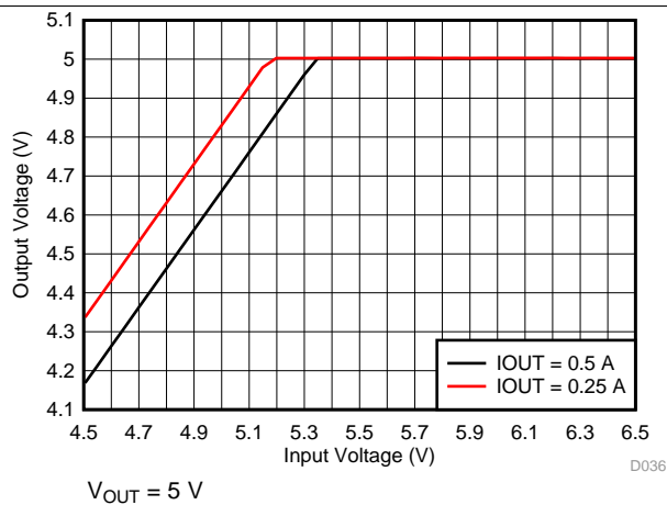
Figure 3. Dropout Voltage
