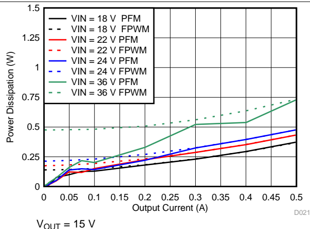
Figure 8. Power Dissipation
