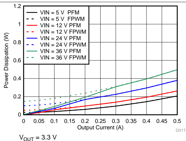
Figure 11. Power Dissipation
