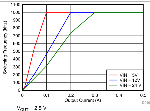
Figure 18. Auto PFM Mode Switching Frequency vs Output Current
