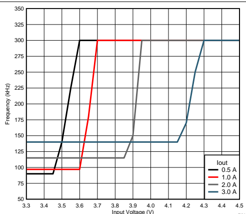
Figure 21. Frequency Foldback
