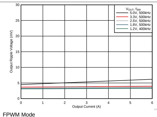
Figure 16. Voltage Ripple vs Output Current
