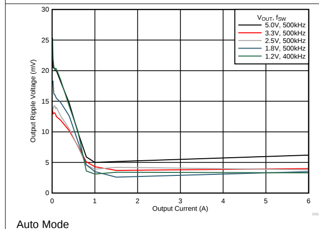
Figure 15. Voltage Ripple vs Output Current
