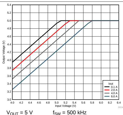
Figure 27. Voltage Dropout
