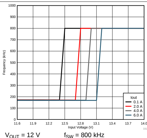
Figure 30. Frequency Foldback
