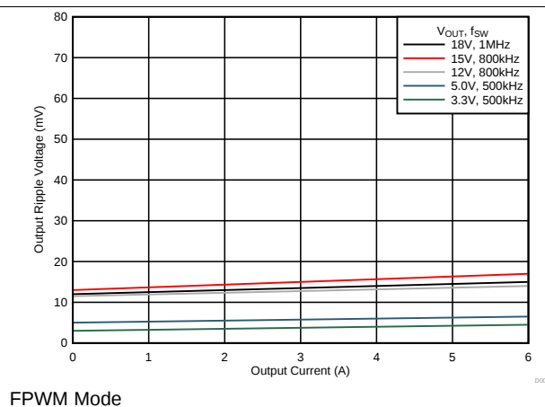
Figure 6. Output Voltage Ripple
