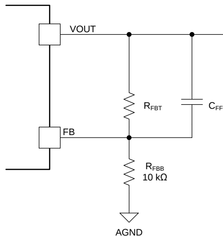
Figure 21. Setting the Output Voltage
