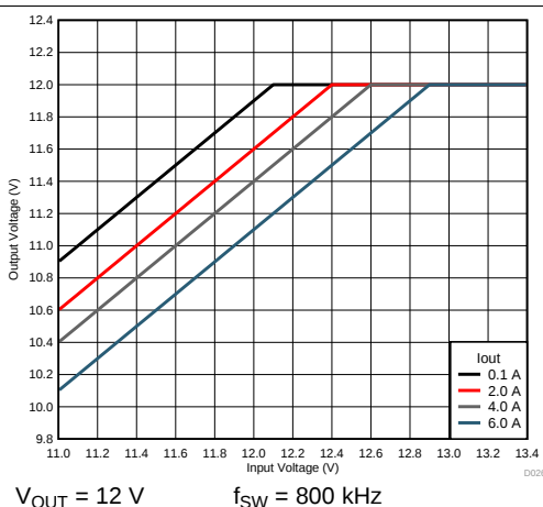
Figure 29. Voltage Dropout
