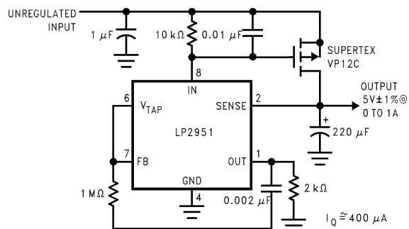
Figure 13. 1A Regulator with 1.2V Dropout
