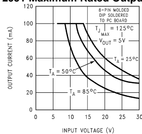
LP2951 Maximum Rated Output Current
