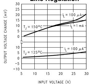
Line Regulation
