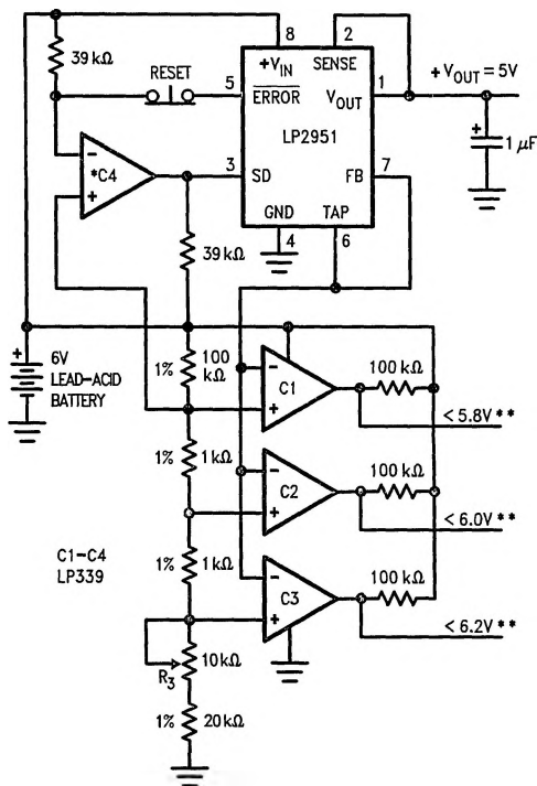
Regulator with State-of-Charge Indicator
