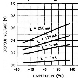
Dropout Voltage
