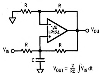
Positive Integrator
